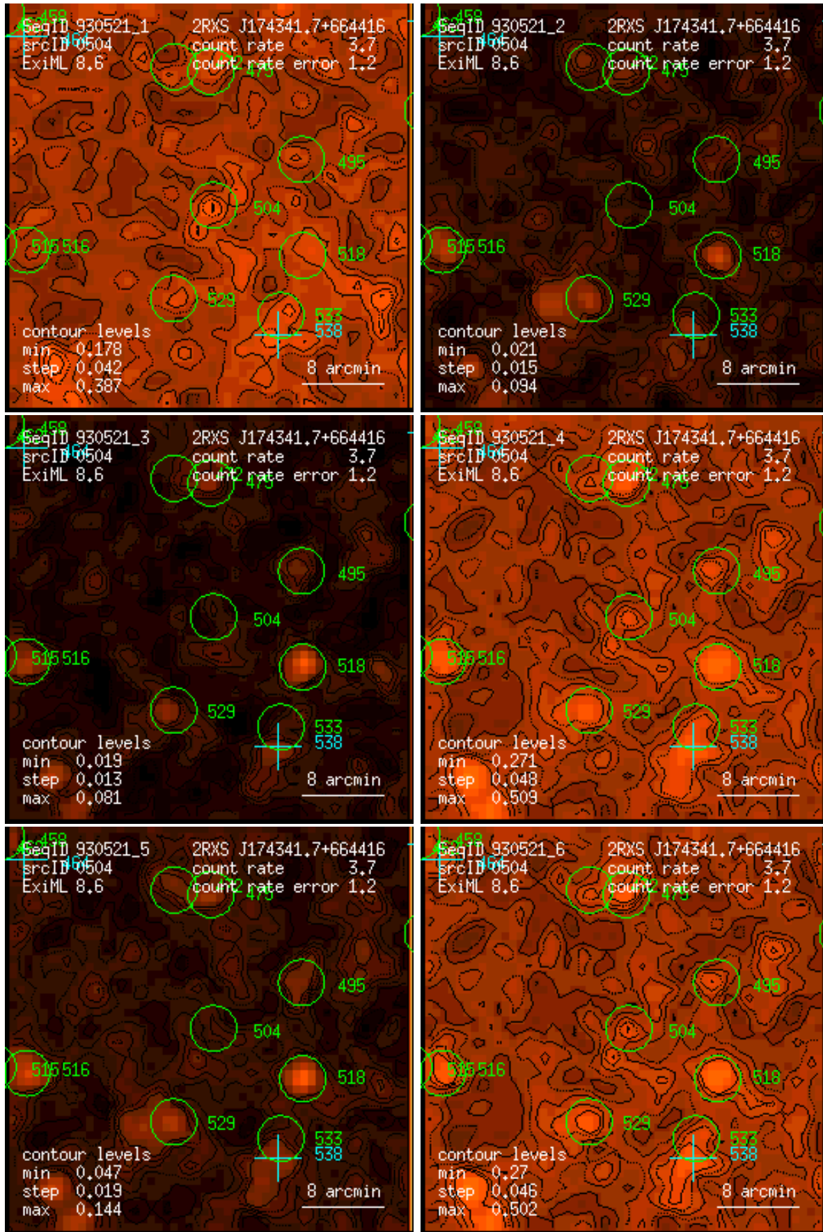
Figure 504: RASS 930521: detection 0504: band rate images, Gaussian filter: (1) PSPC channels 11 – 41, (2) 52 – 90, (3) 91 – 201, (4) 11 – 235, (5) 52 – 201, (6) 11 – 201. Broad band rates in counts/ks. Band rate contour levels in counts/ks/arcmin 2 .
