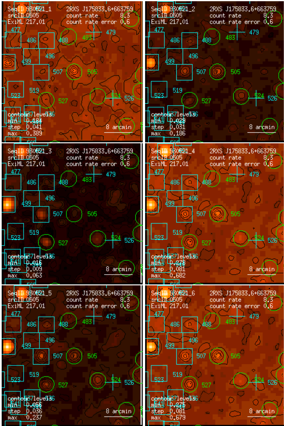
Figure 505: RASS 930521: detection 0505: band rate images, Gaussian filter: (1) PSPC channels 11 – 41, (2) 52 – 90, (3) 91 – 201, (4) 11 – 235, (5) 52 – 201, (6) 11 – 201. Broad band rates in counts/ks. Band rate contour levels in counts/ks/arcmin 2 .
