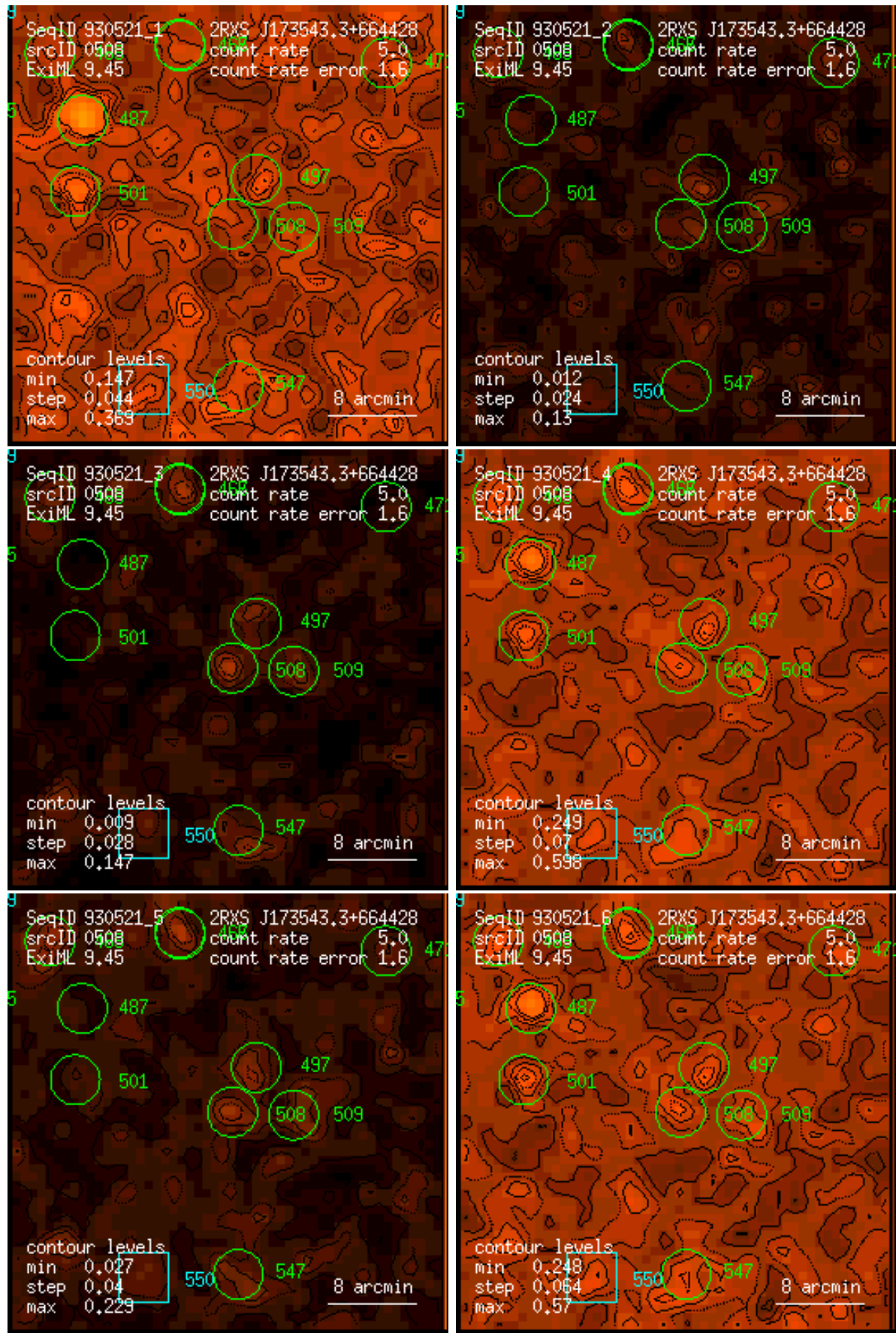
Figure 508: RASS 930521: detection 0508: band rate images, Gaussian filter: (1) PSPC channels 11 – 41, (2) 52 – 90, (3) 91 – 201, (4) 11 – 235, (5) 52 – 201, (6) 11 – 201. Broad band rates in counts/ks. Band rate contour levels in counts/ks/arcmin 2 .
