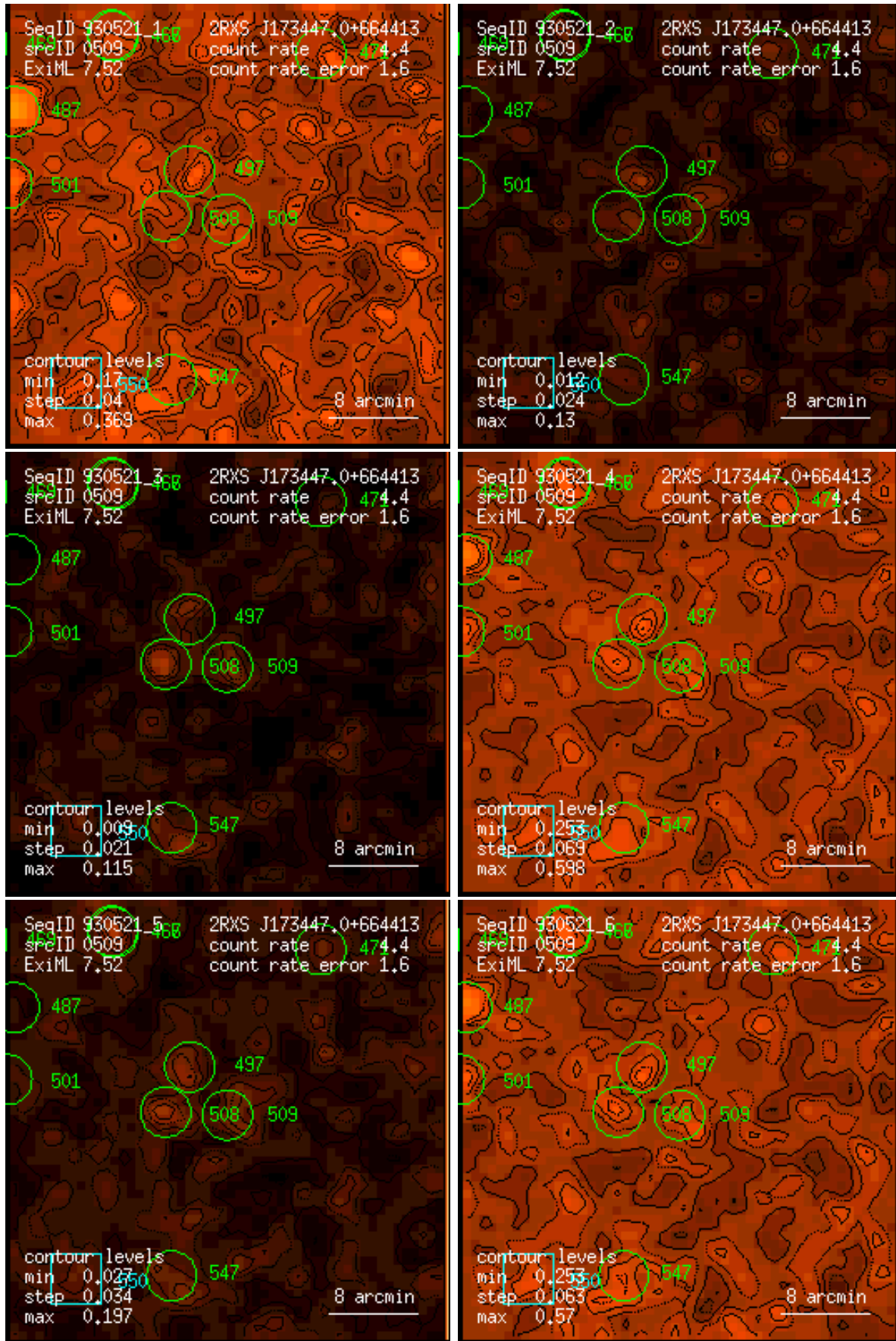
Figure 509: RASS 930521: detection 0509: band rate images, Gaussian filter: (1) PSPC channels 11 – 41, (2) 52 – 90, (3) 91 – 201, (4) 11 – 235, (5) 52 – 201, (6) 11 – 201. Broad band rates in counts/ks. Band rate contour levels in counts/ks/arcmin 2 .
