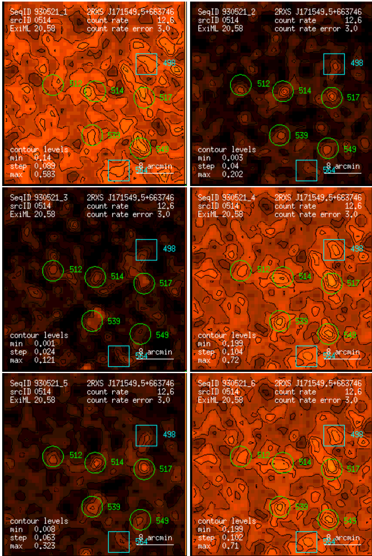
Figure 514: RASS 930521: detection 0514: band rate images, Gaussian filter: (1) PSPC channels 11 – 41, (2) 52 – 90, (3) 91 – 201, (4) 11 – 235, (5) 52 – 201, (6) 11 – 201. Broad band rates in counts/ks. Band rate contour levels in counts/ks/arcmin 2 .
