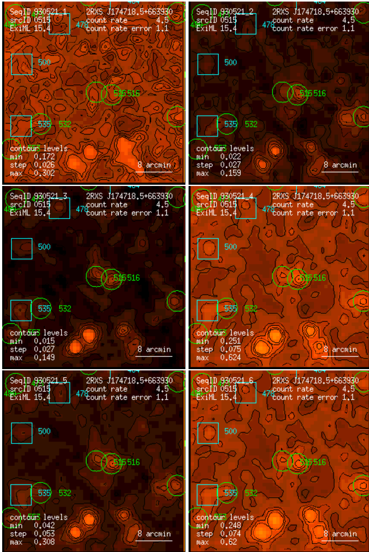
Figure 515: RASS 930521: detection 0515: band rate images, Gaussian filter: (1) PSPC channels 11 – 41, (2) 52 – 90, (3) 91 – 201, (4) 11 – 235, (5) 52 – 201, (6) 11 – 201. Broad band rates in counts/ks. Band rate contour levels in counts/ks/arcmin 2 .
