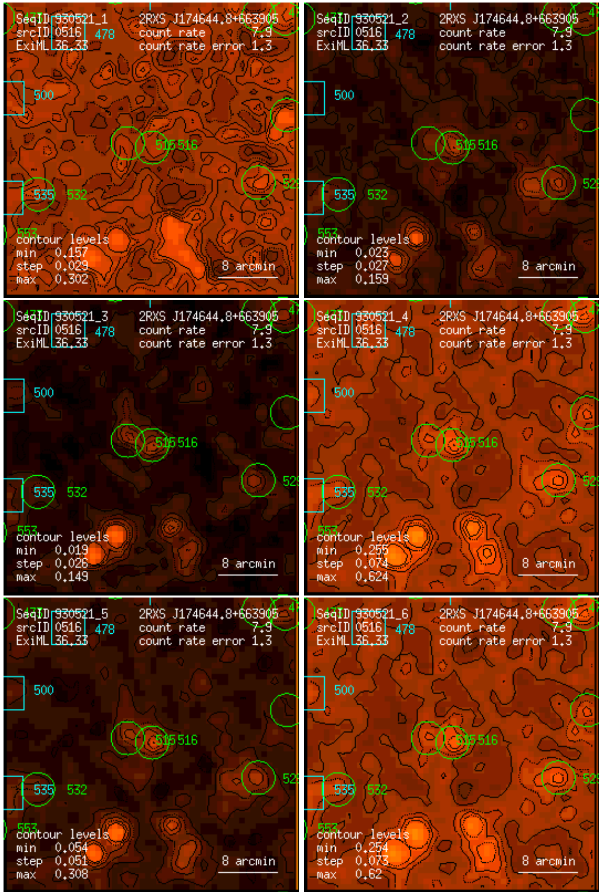
Figure 516: RASS 930521: detection 0516: band rate images, Gaussian filter: (1) PSPC channels 11 – 41, (2) 52 – 90, (3) 91 – 201, (4) 11 – 235, (5) 52 – 201, (6) 11 – 201. Broad band rates in counts/ks. Band rate contour levels in counts/ks/arcmin 2 .
