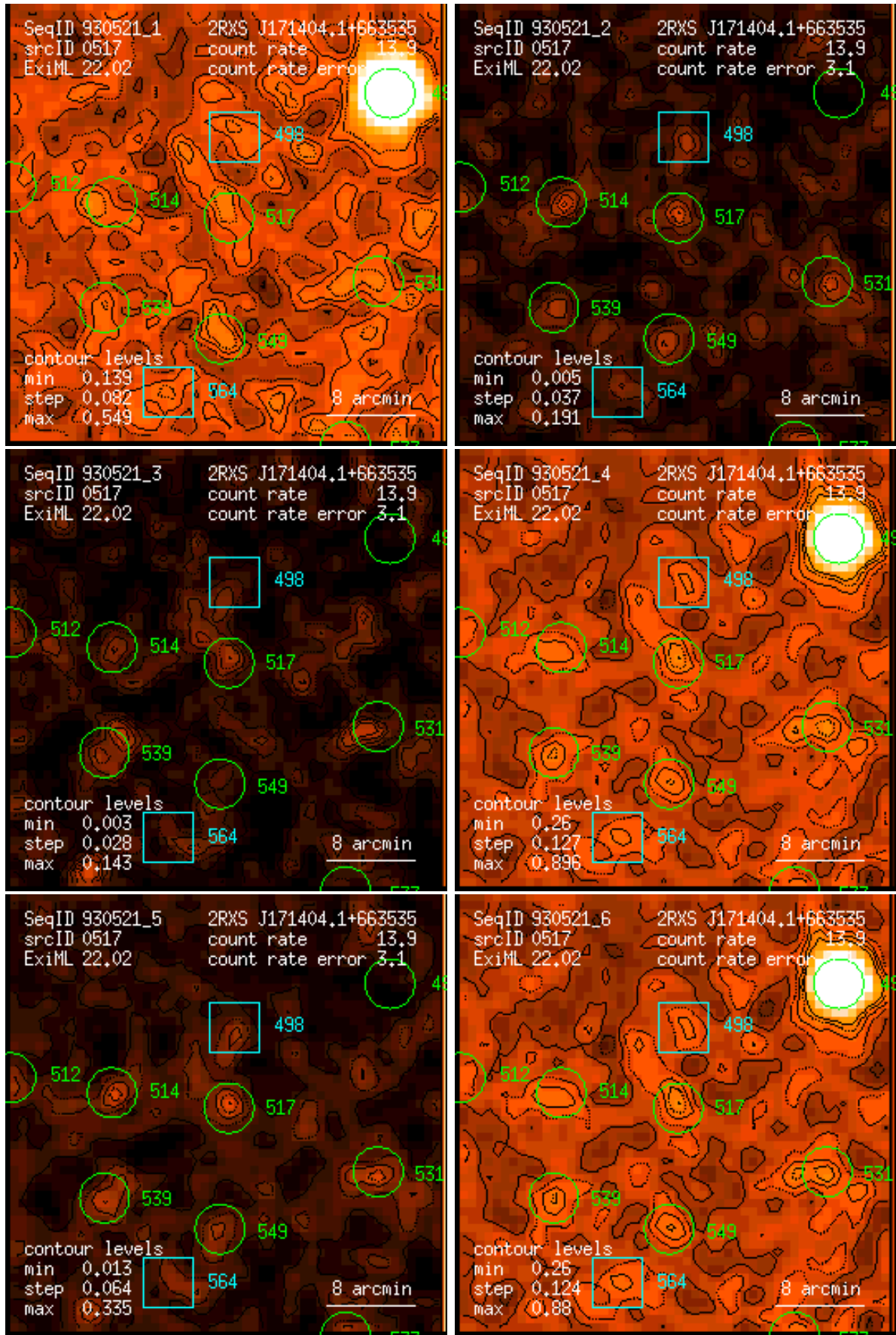
Figure 517: RASS 930521: detection 0517: band rate images, Gaussian filter: (1) PSPC channels 11 – 41, (2) 52 – 90, (3) 91 – 201, (4) 11 – 235, (5) 52 – 201, (6) 11 – 201. Broad band rates in counts/ks. Band rate contour levels in counts/ks/arcmin 2 .
