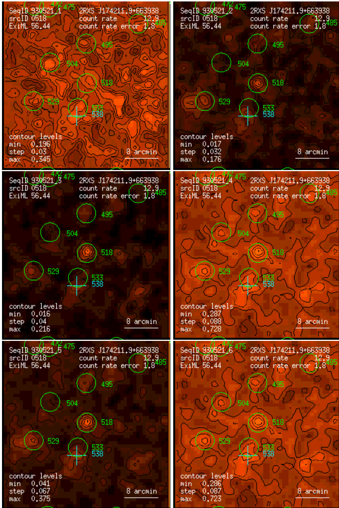
Figure 518: RASS 930521: detection 0518: band rate images, Gaussian filter: (1) PSPC channels 11 – 41, (2) 52 – 90, (3) 91 – 201, (4) 11 – 235, (5) 52 – 201, (6) 11 – 201. Broad band rates in counts/ks. Band rate contour levels in counts/ks/arcmin 2 .
