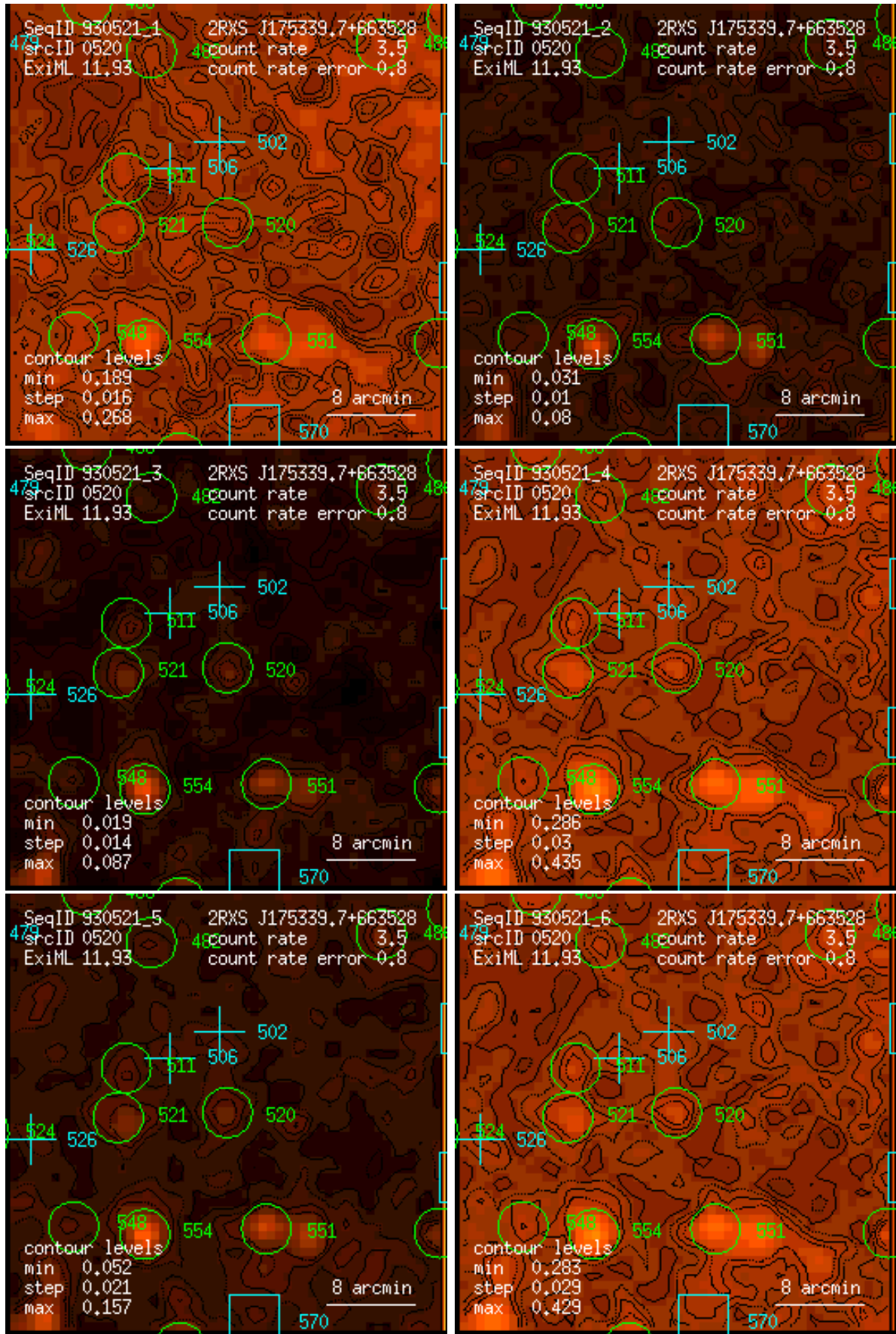
Figure 520: RASS 930521: detection 0520: band rate images, Gaussian filter: (1) PSPC channels 11 – 41, (2) 52 – 90, (3) 91 – 201, (4) 11 – 235, (5) 52 – 201, (6) 11 – 201. Broad band rates in counts/ks. Band rate contour levels in counts/ks/arcmin 2 .
