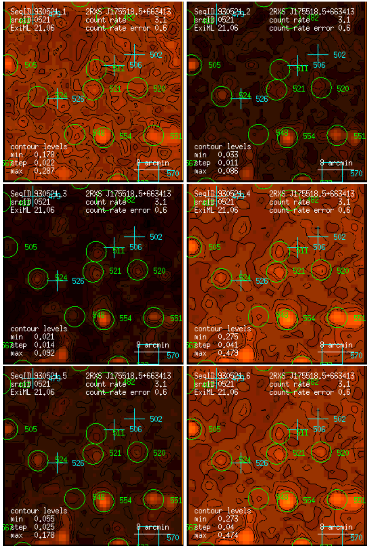
Figure 521: RASS 930521: detection 0521: band rate images, Gaussian filter: (1) PSPPC channels 11 – 41, (2) 52 – 90, (3) 91 – 201, (4) 11 – 235, (5) 52 – 201, (6) 11 – 201. Broad band rates in counts/ks. Band rate contour levels in counts/ks/arcmin 2 .
