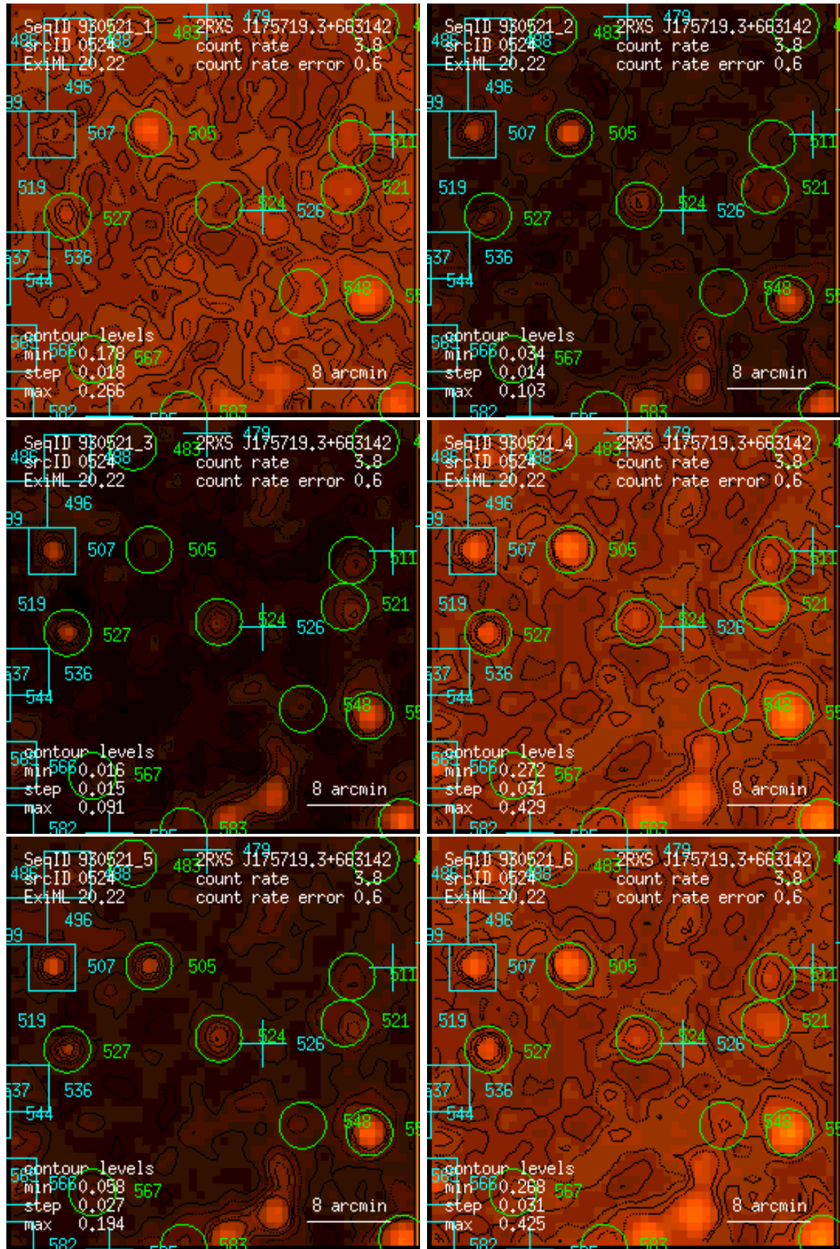
Figure 524: RASS 930521: detection 0524: band rate images, Gaussian filter: (1) PSPC channels 11 – 41, (2) 52 – 90, (3) 91 – 201, (4) 11 – 235, (5) 52 – 201, (6) 11 – 201. Broad band rates in counts/ks. Band rate contour levels in counts/ks/arcmin 2 .
