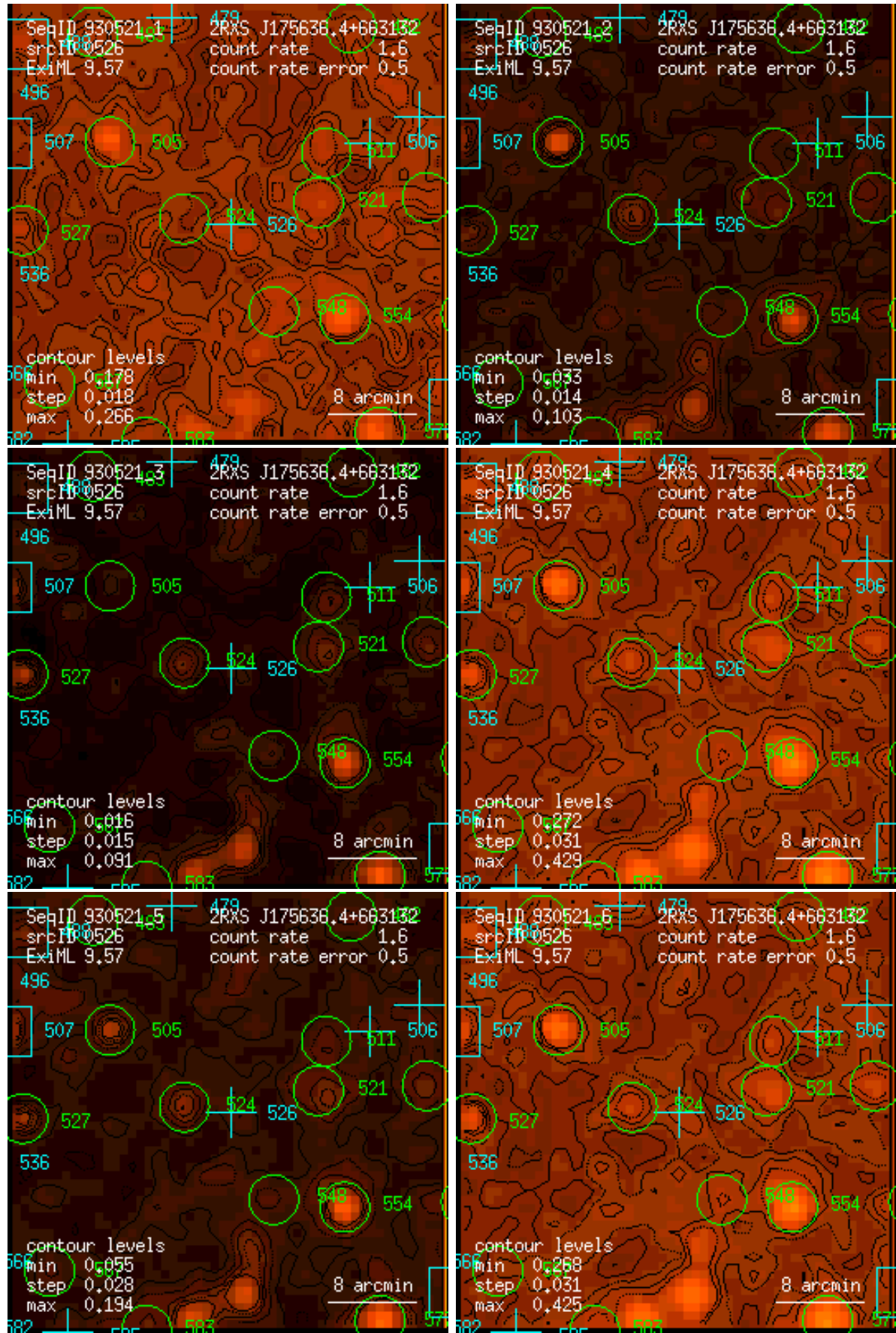
Figure 526: RASS 930521: detection 0526: band rate images, Gaussian filter: (1) PSPC channels 11 – 41, (2) 52 – 90, (3) 91 – 201, (4) 11 – 235, (5) 52 – 201, (6) 11 – 201. Broad band rates in counts/ks. Band rate contour levels in counts/ks/arcmin 2 .
