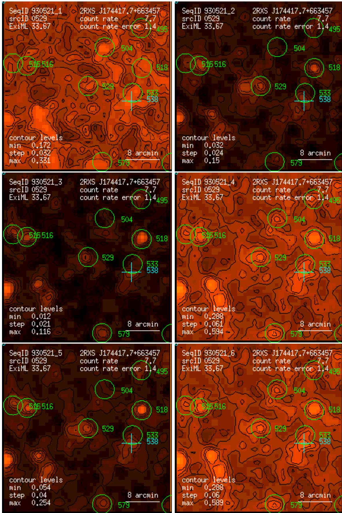
Figure 529: RASS 930521: detection 0529: band rate images, Gaussian filter: (1) PSPC channels 11 – 41, (2) 52 – 90, (3) 91 – 201, (4) 11 – 235, (5) 52 – 201, (6) 11 – 201. Broad band rates in counts/ks. Band rate contour levels in counts/ks/arcmin 2 .
