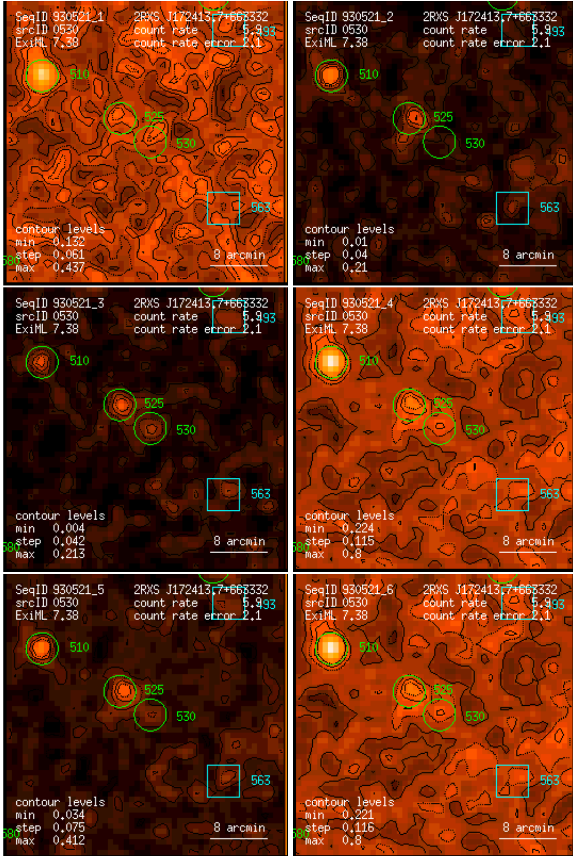
Figure 530: RASS 930521: detection 0530: band rate images, Gaussian filter: (1) PSPC channels 11 – 41, (2) 52 – 90, (3) 91 – 201, (4) 11 – 235, (5) 52 – 201, (6) 11 – 201. Broad band rates in counts/ks. Band rate contour levels in counts/ks/arcmin 2 .
