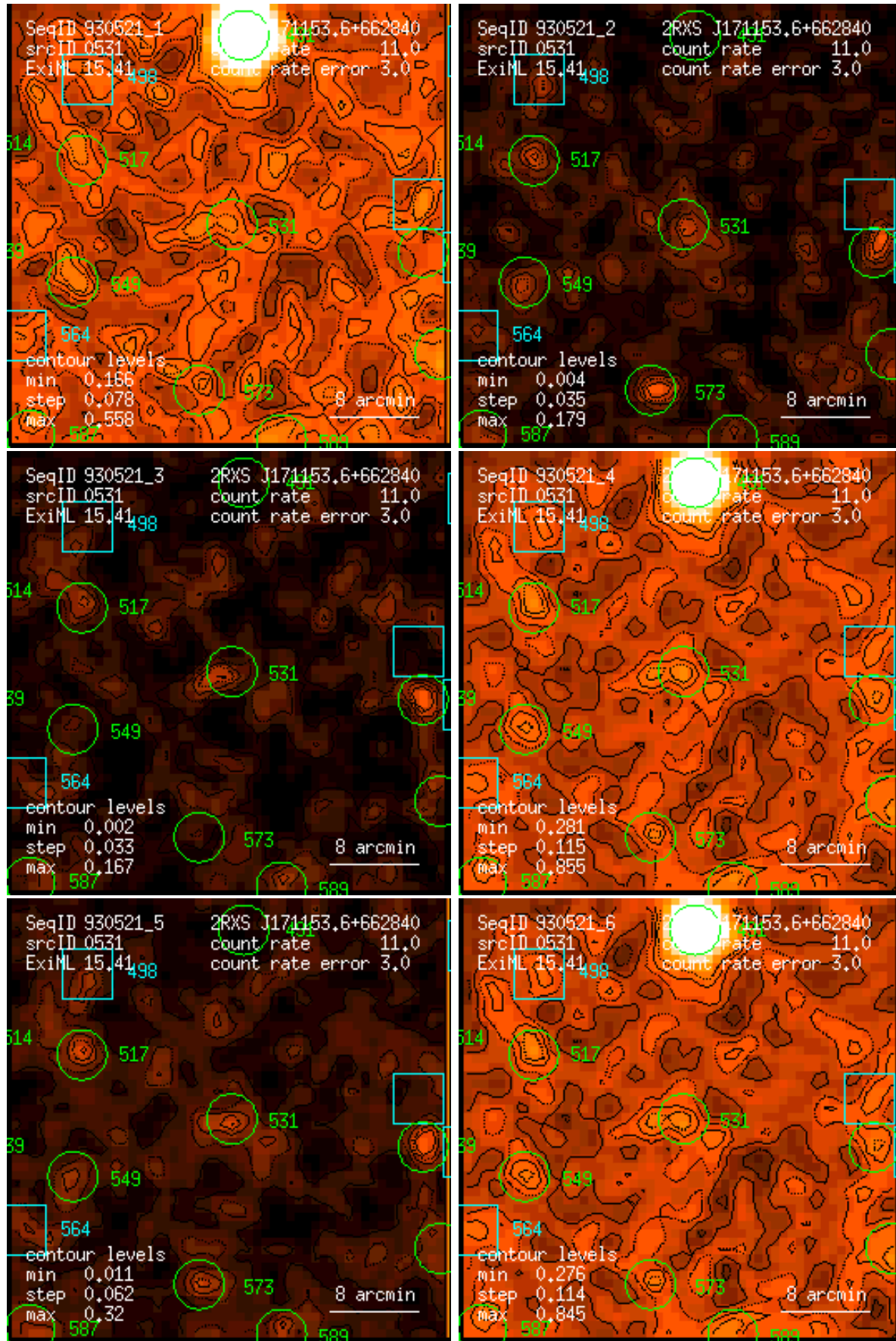
Figure 531: RASS 930521: detection 0531: band rate images, Gaussian filter: (1) PSPC channels 11 – 41, (2) 52 – 90, (3) 91 – 201, (4) 11 – 235, (5) 52 – 201, (6) 11 – 201. Broad band rates in counts/ks. Band rate contour levels in counts/ks/arcmin 2 .
