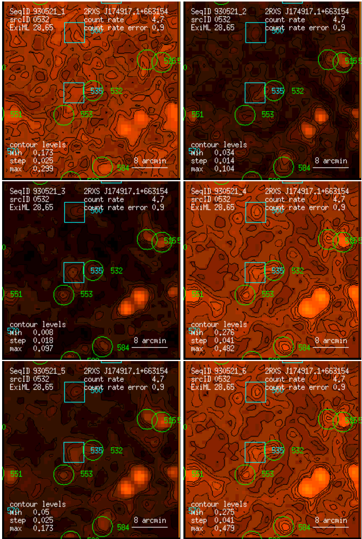
Figure 532: RASS 930521: detection 0532: band rate images, Gaussian filter: (1) PSPC channels 11 – 41, (2) 52 – 90, (3) 91 – 201, (4) 11 – 235, (5) 52 – 201, (6) 11 – 201. Broad band rates in counts/ks. Band rate contour levels in counts/ks/arcmin 2 .
