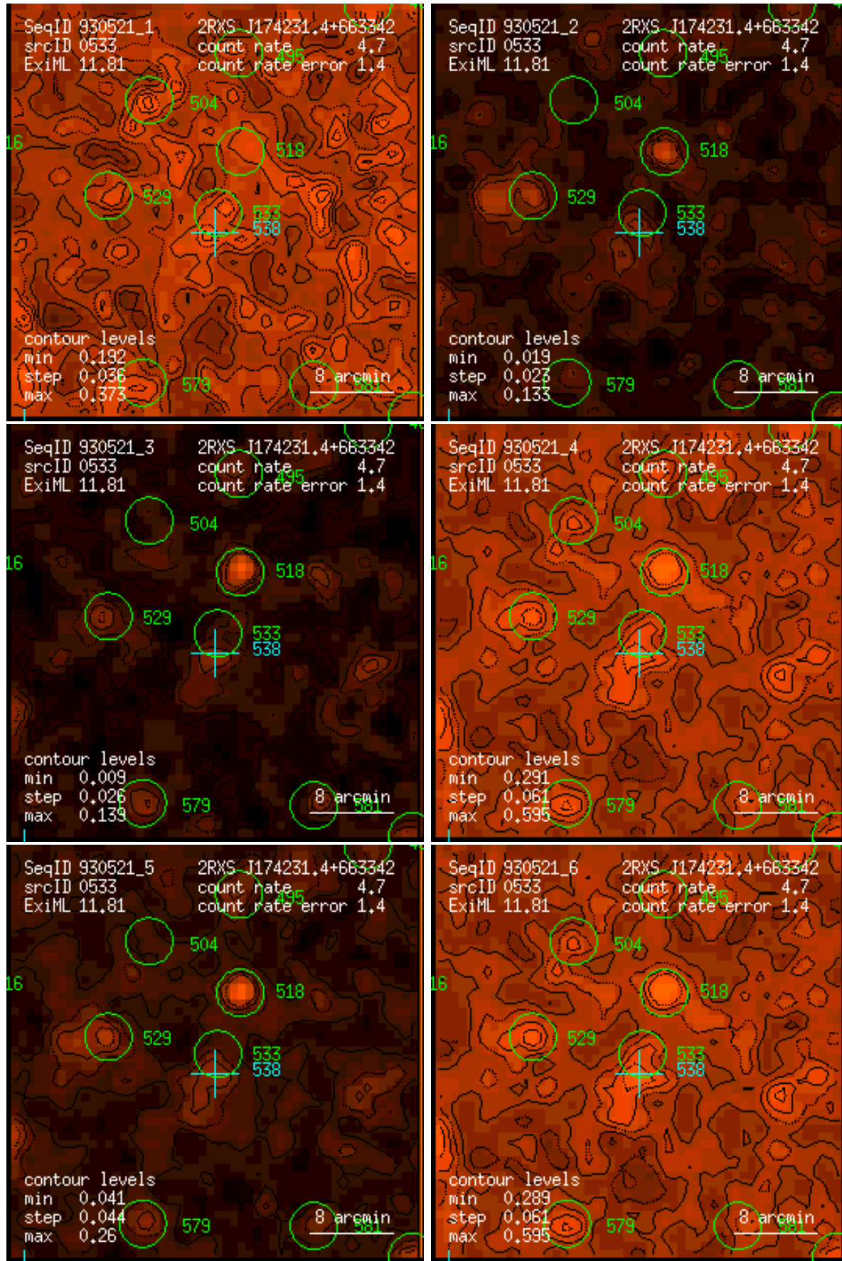
Figure 533: RASS 930521: detection 0533: band rate images, Gaussian filter: (1) PSPC channels 11 – 41, (2) 52 – 90, (3) 91 – 201, (4) 11 – 235, (5) 52 – 201, (6) 11 – 201. Broad band rates in counts/ks. Band rate contour levels in counts/ks/arcmin 2 .
