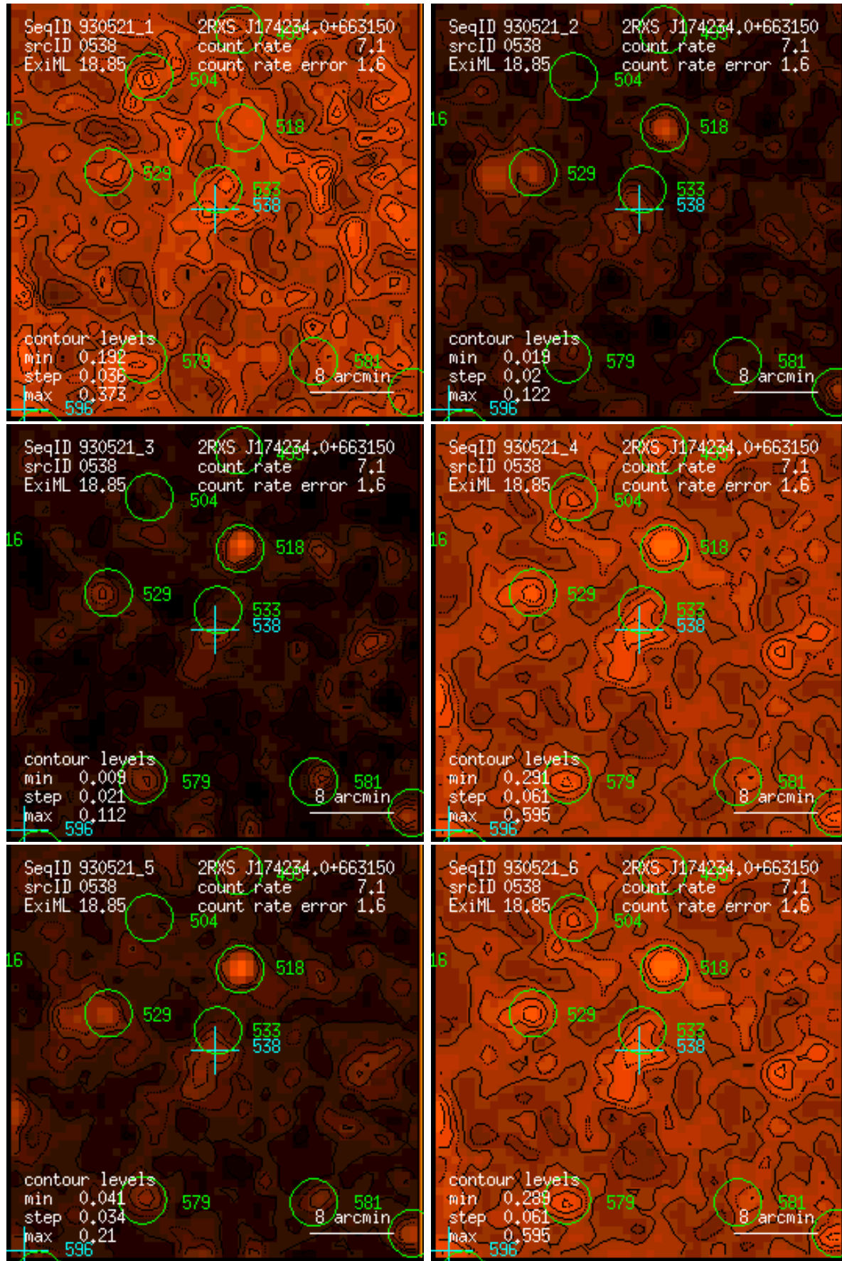
Figure 538: RASS 930521: detection 0538: band rate images, Gaussian filter: (1) PSPC channels 11 – 41, (2) 52 – 90, (3) 91 – 201, (4) 11 – 235, (5) 52 – 201, (6) 11 – 201. Broad band rates in counts/ks. Band rate contour levels in counts/ks/arcmin 2 .
