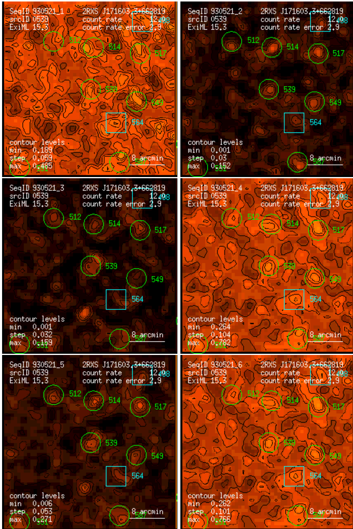
Figure 539: RASS 930521: detection 0539: band rate images, Gaussian filter: (1) PSPC channels 11 – 41, (2) 52 – 90, (3) 91 – 201, (4) 11 – 235, (5) 52 – 201, (6) 11 – 201. Broad band rates in counts/ks. Band rate contour levels in counts/ks/arcmin 2 .
