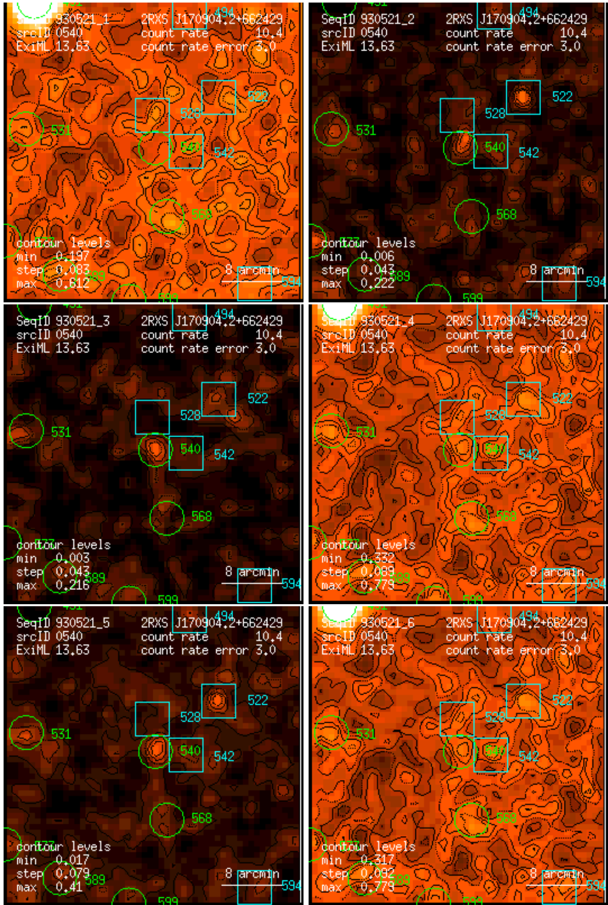
Figure 540: RASS 930521: detection 0540: band rate images, Gaussian filter: (1) PSPC channels 11 – 41, (2) 52 – 90, (3) 91 – 201, (4) 11 – 235, (5) 52 – 201, (6) 11 – 201. Broad band rates in counts/ks. Band rate contour levels in counts/ks/arcmin 2 .
