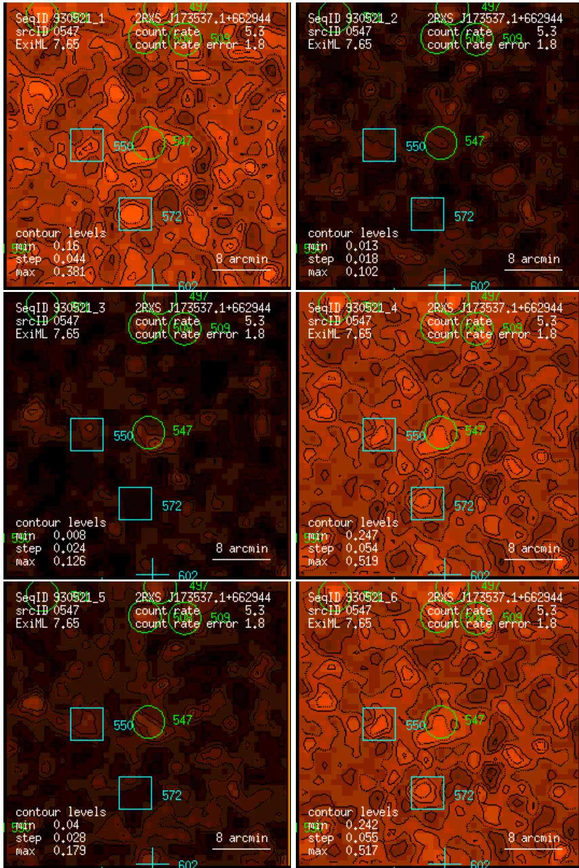
Figure 547: RASS 930521: detection 0547: band rate images, Gaussian filter: (1) PSPC channels 11 – 41, (2) 52 – 90, (3) 91 – 201, (4) 11 – 235, (5) 52 – 201, (6) 11 – 201. Broad band rates in counts/ks. Band rate contour levels in counts/ks/arcmin 2 .
