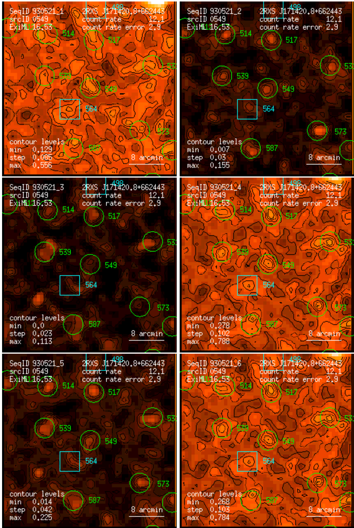
Figure 549: RASS 930521: detection 0549: band rate images, Gaussian filter: (1) PSPC channels 11 – 41, (2) 52 – 90, (3) 91 – 201, (4) 11 – 235, (5) 52 – 201, (6) 11 – 201. Broad band rates in counts/ks. Band rate contour levels in counts/ks/arcmin 2 .
