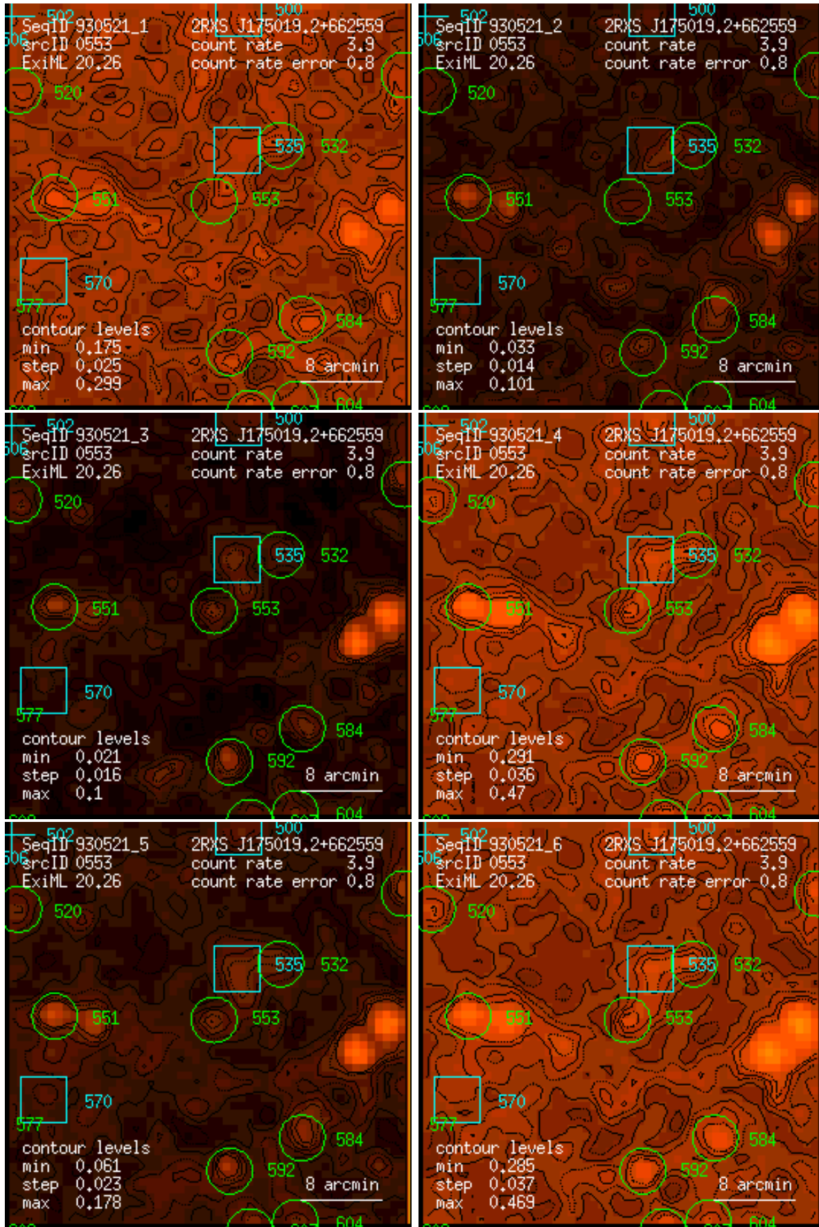
Figure 553: RASS 930521: detection 0553: band rate images, Gaussian filter: (1) PSPC channels 11 – 41, (2) 52 – 90, (3) 91 – 201, (4) 11 – 235, (5) 52 – 201, (6) 11 – 201. Broad band rates in counts/ks. Band rate contour levels in counts/ks/arcmin 2 .
