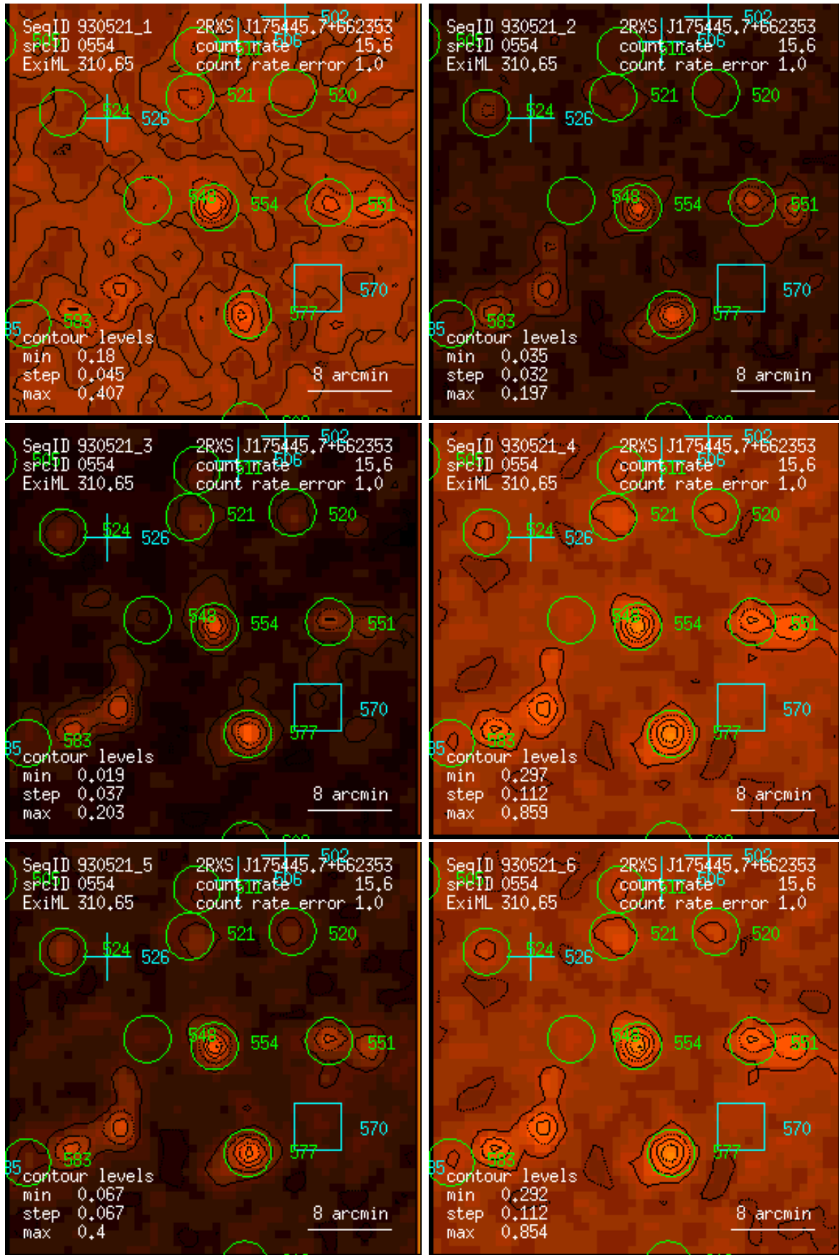
Figure 554: RASS 930521: detection 0554: band rate images, Gaussian filter: (1) PSPC channels 11 – 41, (2) 52 – 90, (3) 91 – 201, (4) 11 – 235, (5) 52 – 201, (6) 11 – 201. Broad band rates in counts/ks. Band rate contour levels in counts/ks/arcmin 2 .
