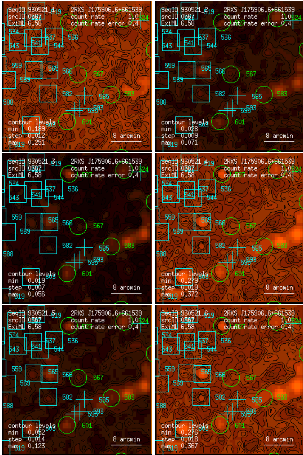
Figure 567: RASS 930521: detection 0567: band rate images, Gaussian filter: (1) PSPC channels 11 – 41, (2) 52 – 90, (3) 91 – 201, (4) 11 – 235, (5) 52 – 201, (6) 11 – 201. Broad band rates in counts/ks. Band rate contour levels in counts/ks/arcmin 2 .
