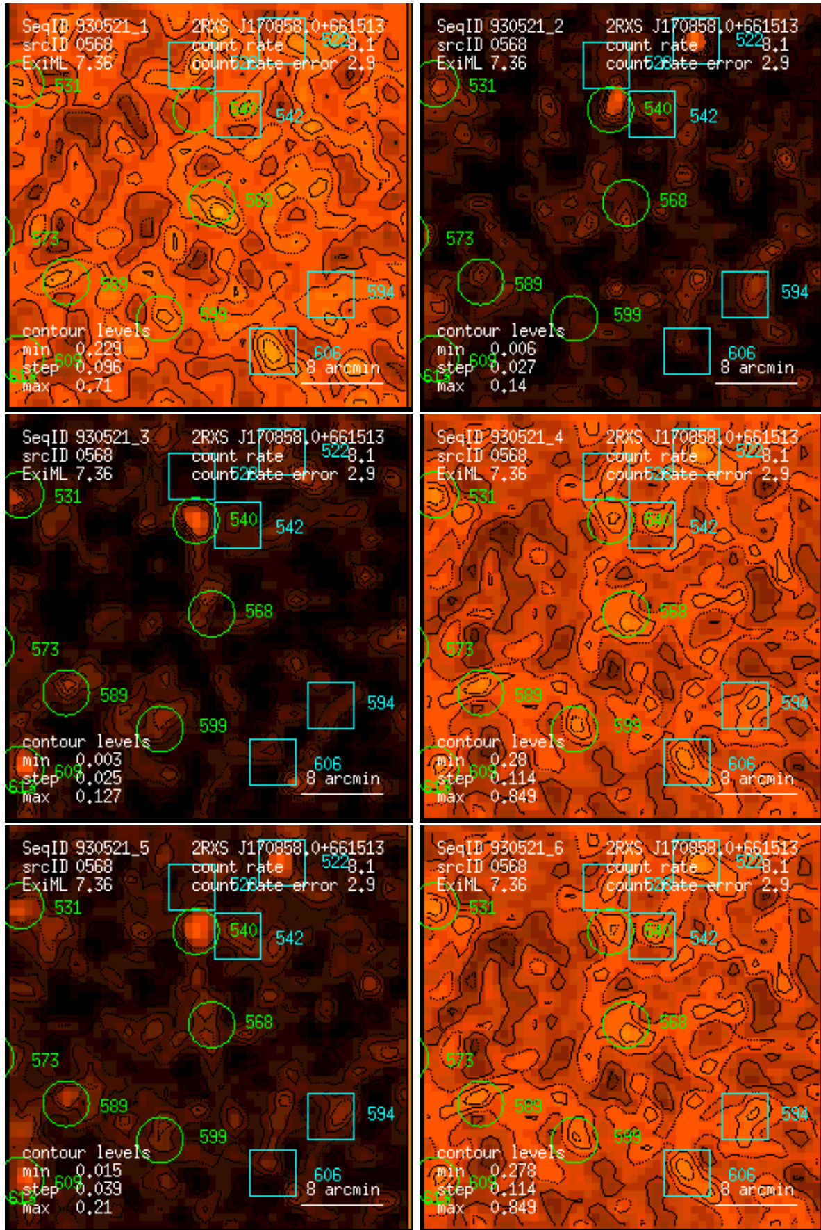
Figure 568: RASS 930521: detection 0568: band rate images, Gaussian filter: (1) PSPC channels 11 – 41, (2) 52 – 90, (3) 91 – 201, (4) 11 – 235, (5) 52 – 201, (6) 11 – 201. Broad band rates in counts/ks. Band rate contour levels in counts/ks/arcmin 2 .
