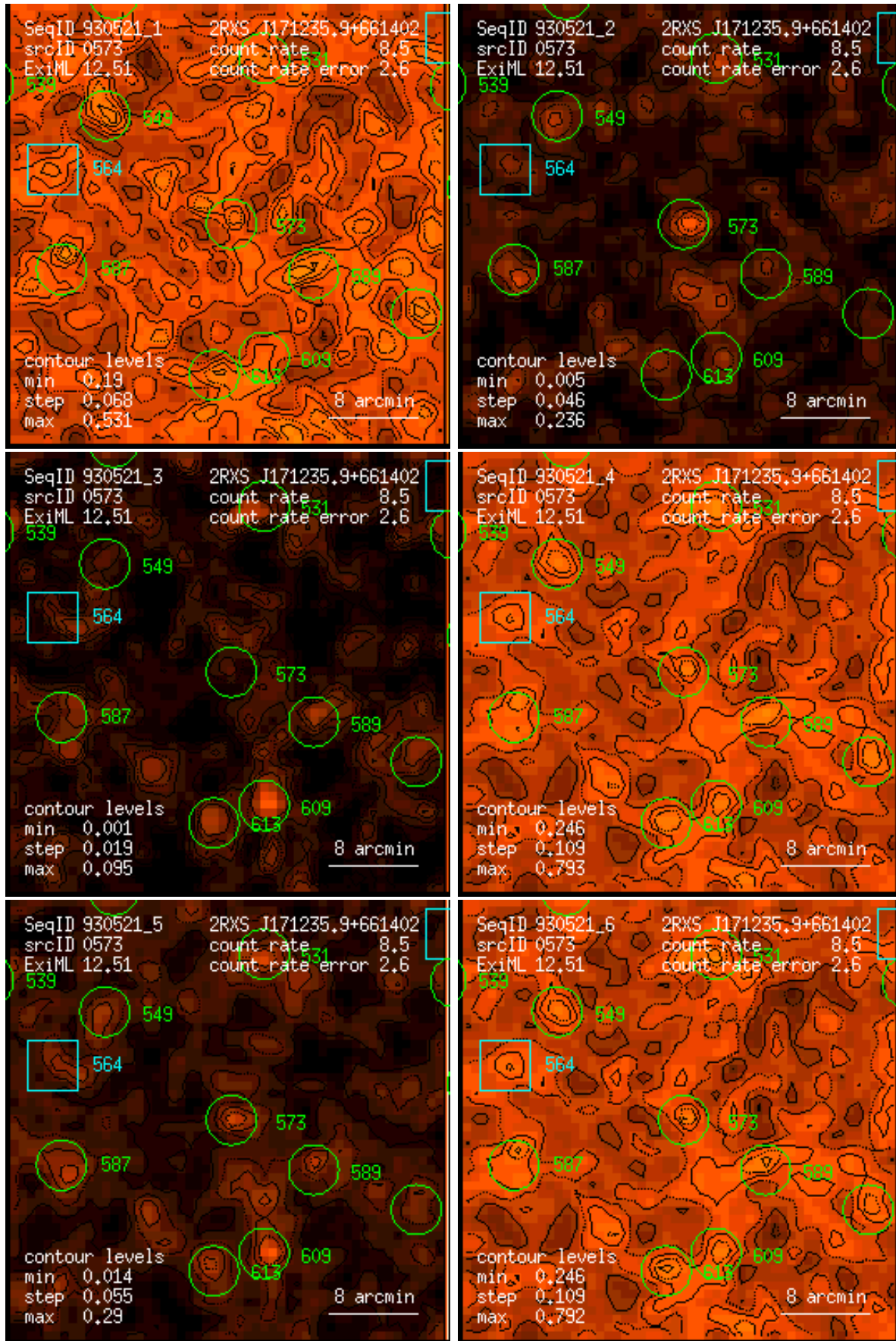
Figure 573: RASS 930521: detection 0573: band rate images, Gaussian filter: (1) PSPC channels 11 – 41, (2) 52 – 90, (3) 91 – 201, (4) 11 – 235, (5) 52 – 201, (6) 11 – 201. Broad band rates in counts/ks. Band rate contour levels in counts/ks/arcmin 2 .
