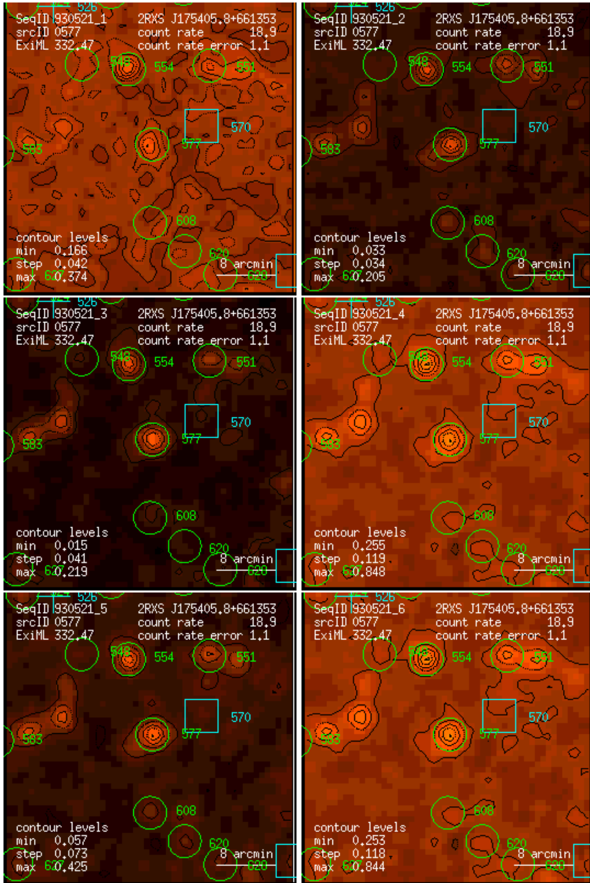
Figure 577: RASS 930521: detection 0577: band rate images, Gaussian filter: (1) PSPC channels 11 – 41, (2) 52 – 90, (3) 91 – 201, (4) 11 – 235, (5) 52 – 201, (6) 11 – 201. Broad band rates in counts/ks. Band rate contour levels in counts/ks/arcmin 2 .
