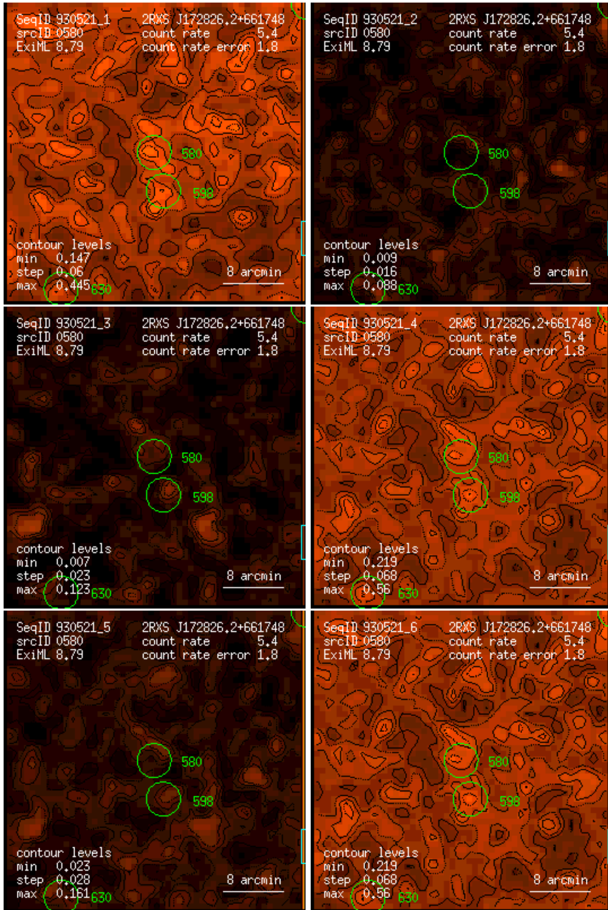
Figure 580: RASS 930521: detection 0580: band rate images, Gaussian filter: (1) PSPC channels 11 – 41, (2) 52 – 90, (3) 91 – 201, (4) 11 – 235, (5) 52 – 201, (6) 11 – 201. Broad band rates in counts/ks. Band rate contour levels in counts/ks/arcmin 2 .
