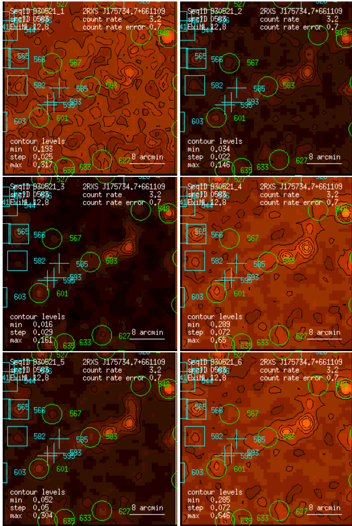
Figure 583: RASS 930521: detection 0583: band rate images, Gaussian filter: (1) PSPC channels 11 – 41, (2) 52 – 90, (3) 91 – 201, (4) 11 – 235, (5) 52 – 201, (6) 11 – 201. Broad band rates in counts/ks. Band rate contour levels in counts/ks/arcmin 2 .
