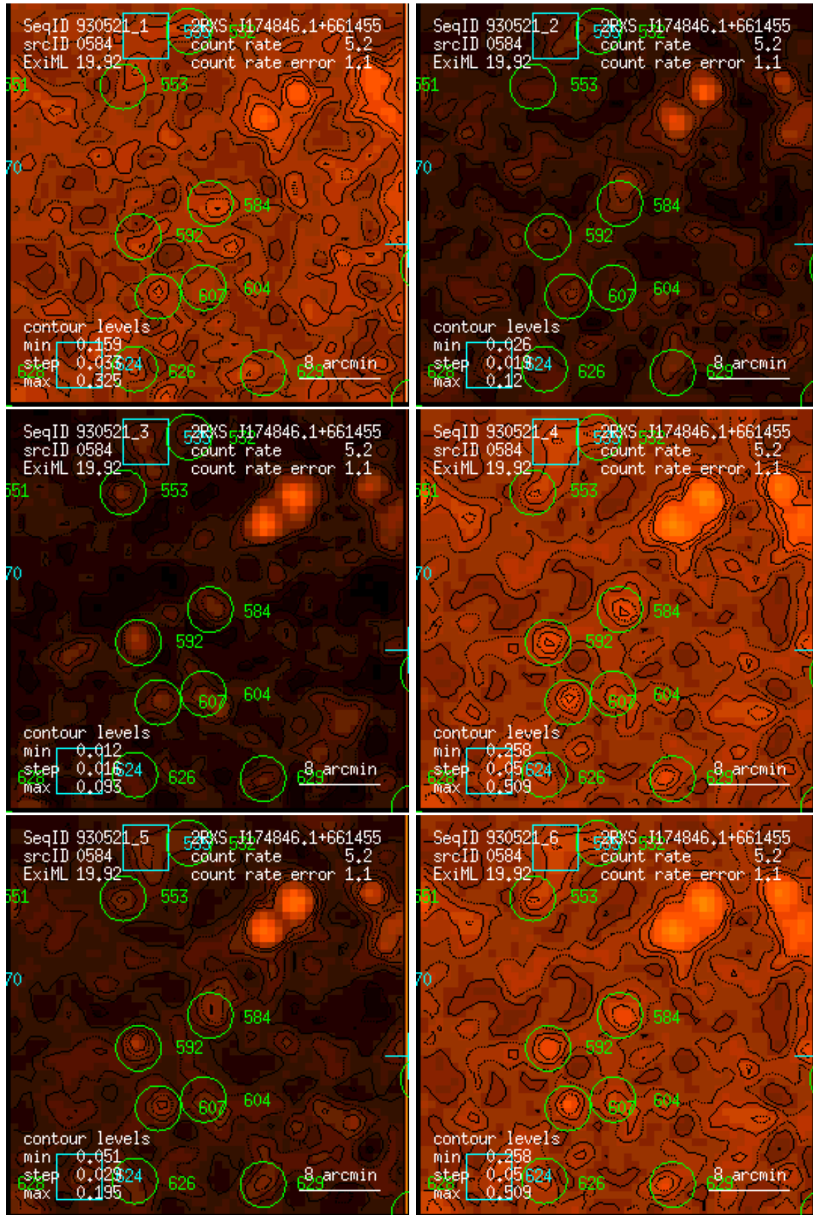
Figure 584: RASS 930521: detection 0584: band rate images, Gaussian filter: (1) PSPC channels 11 – 41, (2) 52 – 90, (3) 91 – 201, (4) 11 – 235, (5) 52 – 201, (6) 11 – 201. Broad band rates in counts/ks. Band rate contour levels in counts/ks/arcmin 2 .
