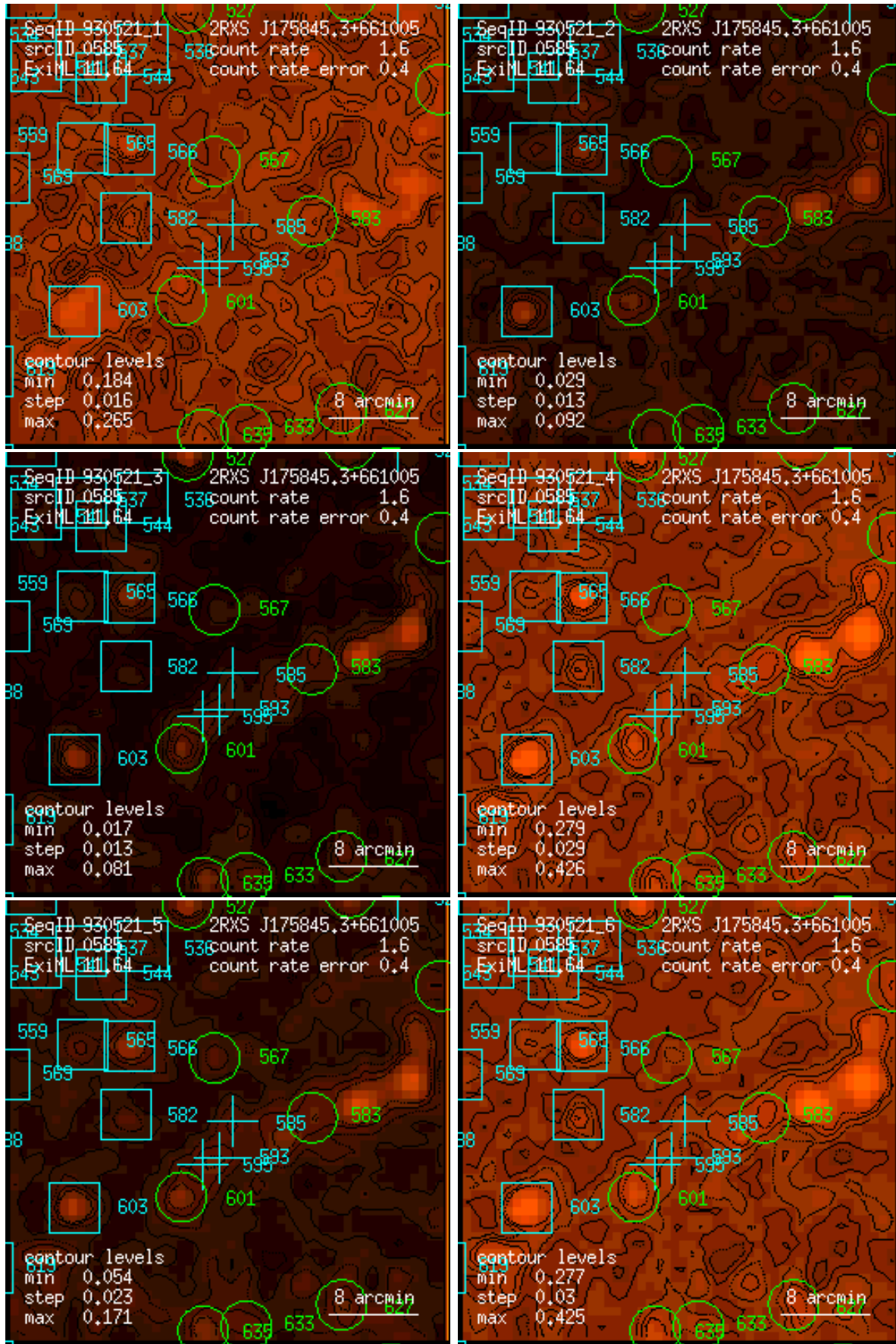
Figure 585: RASS 930521: detection 0585: band rate images, Gaussian filter: (1) PSPC channels 11 – 41, (2) 52 – 90, (3) 91 – 201, (4) 11 – 235, (5) 52 – 201, (6) 11 – 201. Broad band rates in counts/ks. Band rate contour levels in counts/ks/arcmin 2 .
