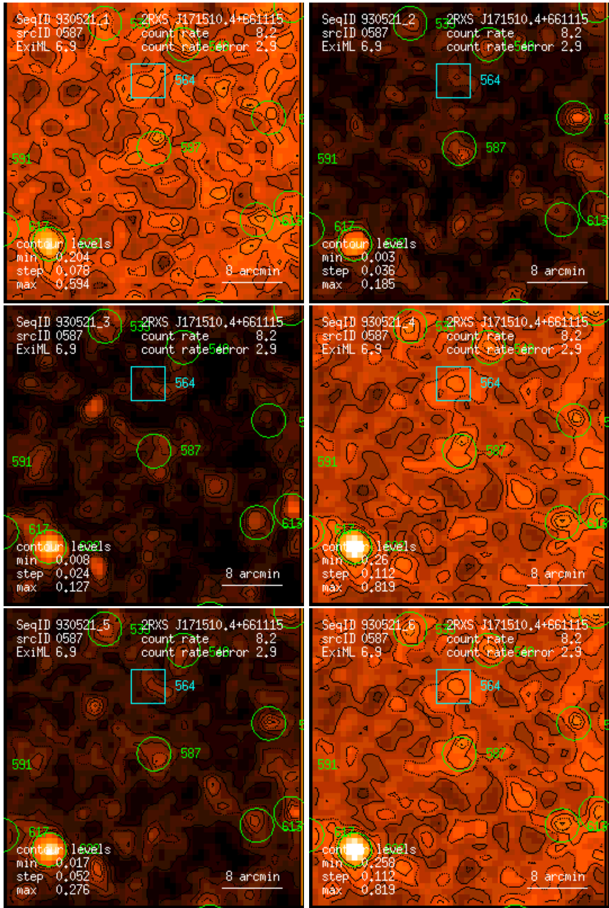
Figure 587: RASS 930521: detection 0587: band rate images, Gaussian filter: (1) PSPC channels 11 – 41, (2) 52 – 90, (3) 91 – 201, (4) 11 – 235, (5) 52 – 201, (6) 11 – 201. Broad band rates in counts/ks. Band rate contour levels in counts/ks/arcmin 2 .
