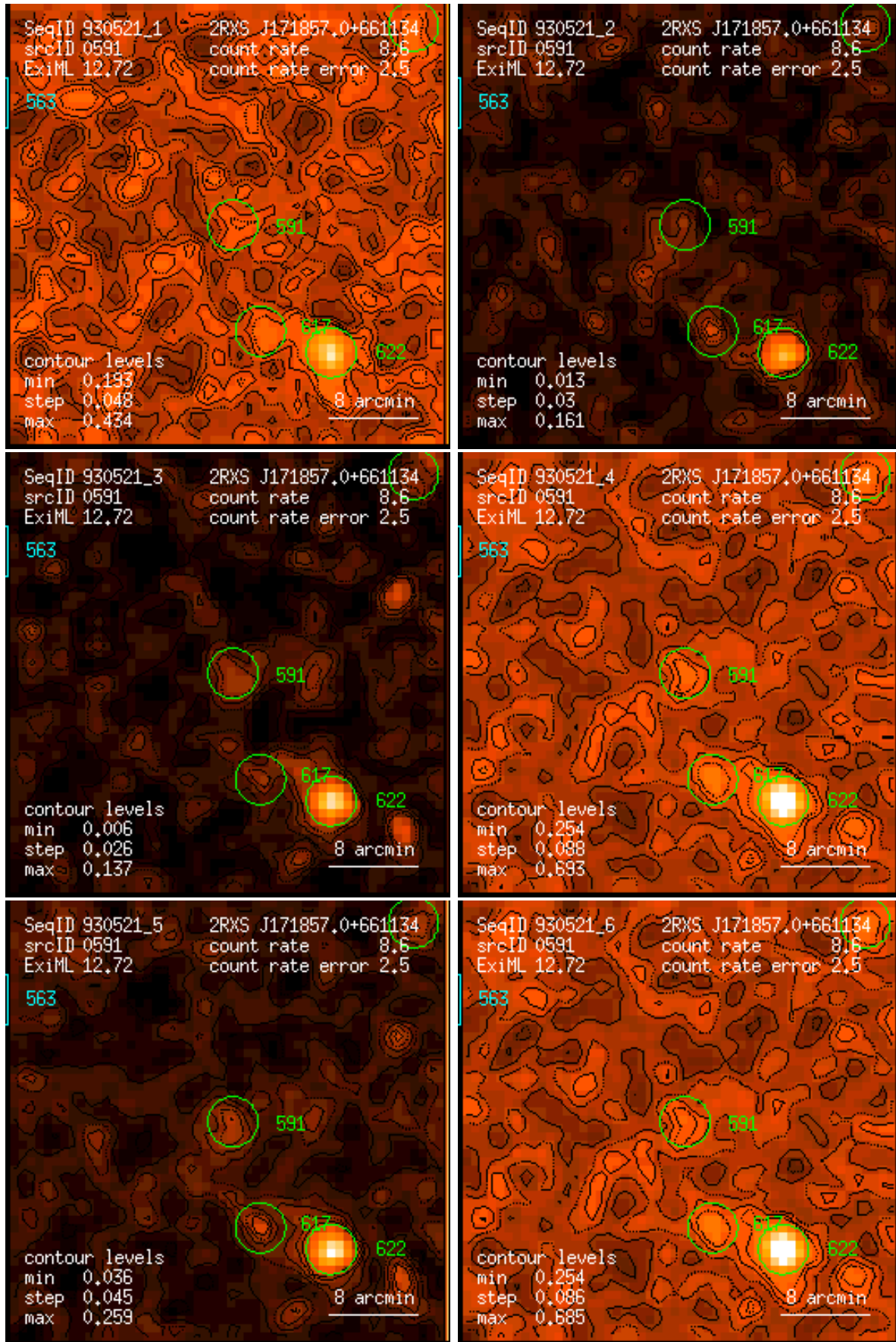
Figure 591: RASS 930521: detection 0591: band rate images, Gaussian filter: (1) PSPC channels 11 – 41, (2) 52 – 90, (3) 91 – 201, (4) 11 – 235, (5) 52 – 201, (6) 11 – 201. Broad band rates in counts/ks. Band rate contour levels in counts/ks/arcmin 2 .
