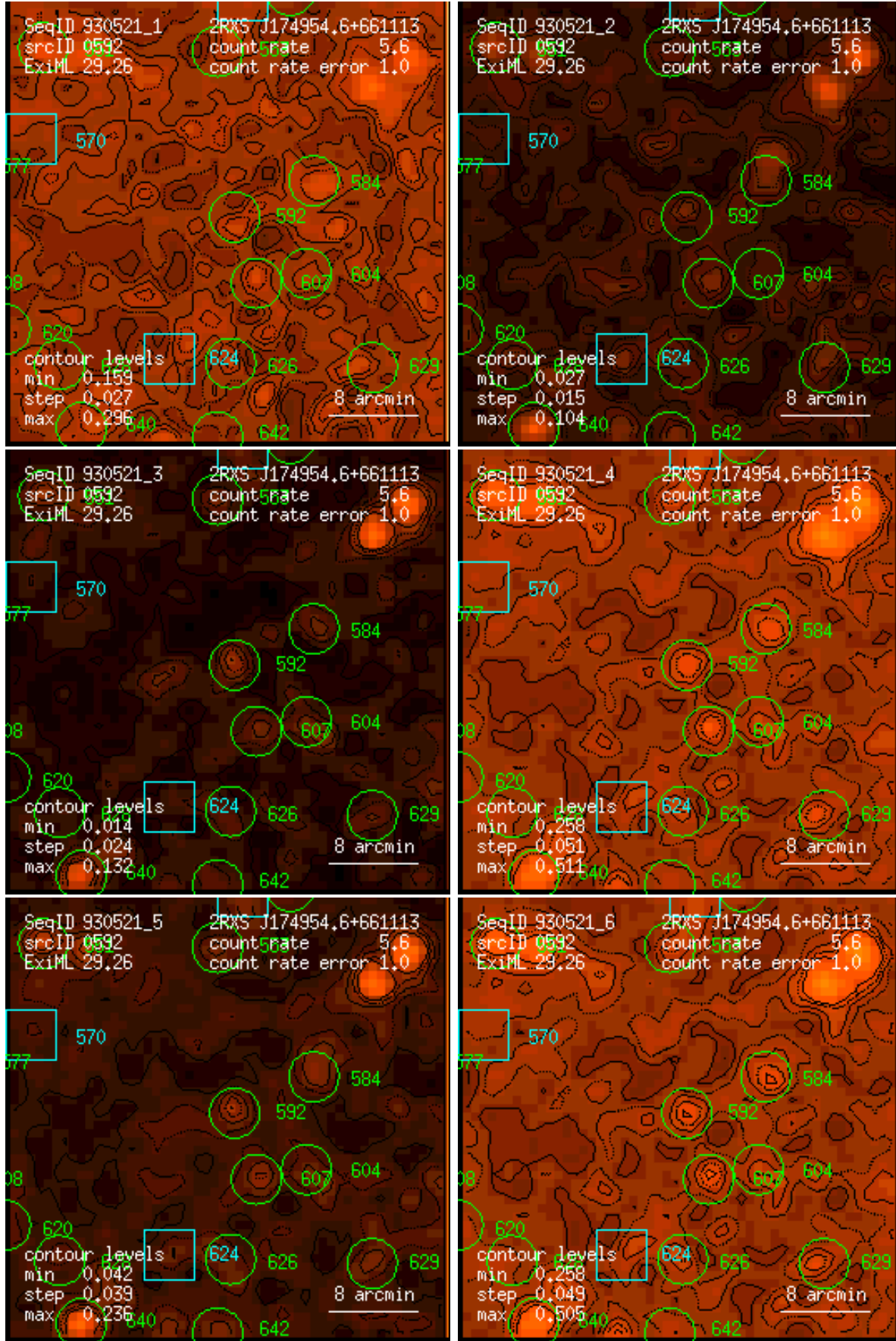
Figure 592: RASS 930521: detection 0592: band rate images, Gaussian filter: (1) PSPC channels 11 – 41, (2) 52 – 90, (3) 91 – 201, (4) 11 – 235, (5) 52 – 201, (6) 11 – 201. Broad band rates in counts/ks. Band rate contour levels in counts/ks/arcmin 2 .
