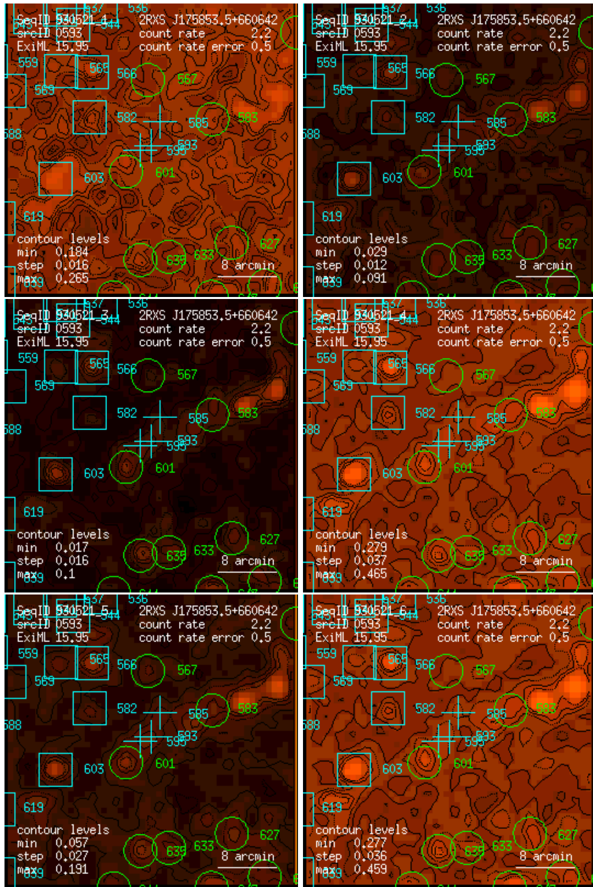
Figure 593: RASS 930521: detection 0593: band rate images, Gaussian filter: (1) PSPC channels 11 – 41, (2) 52 – 90, (3) 91 – 201, (4) 11 – 235, (5) 52 – 201, (6) 11 – 201. Broad band rates in counts/ks. Band rate contour levels in counts/ks/arcmin 2 .
