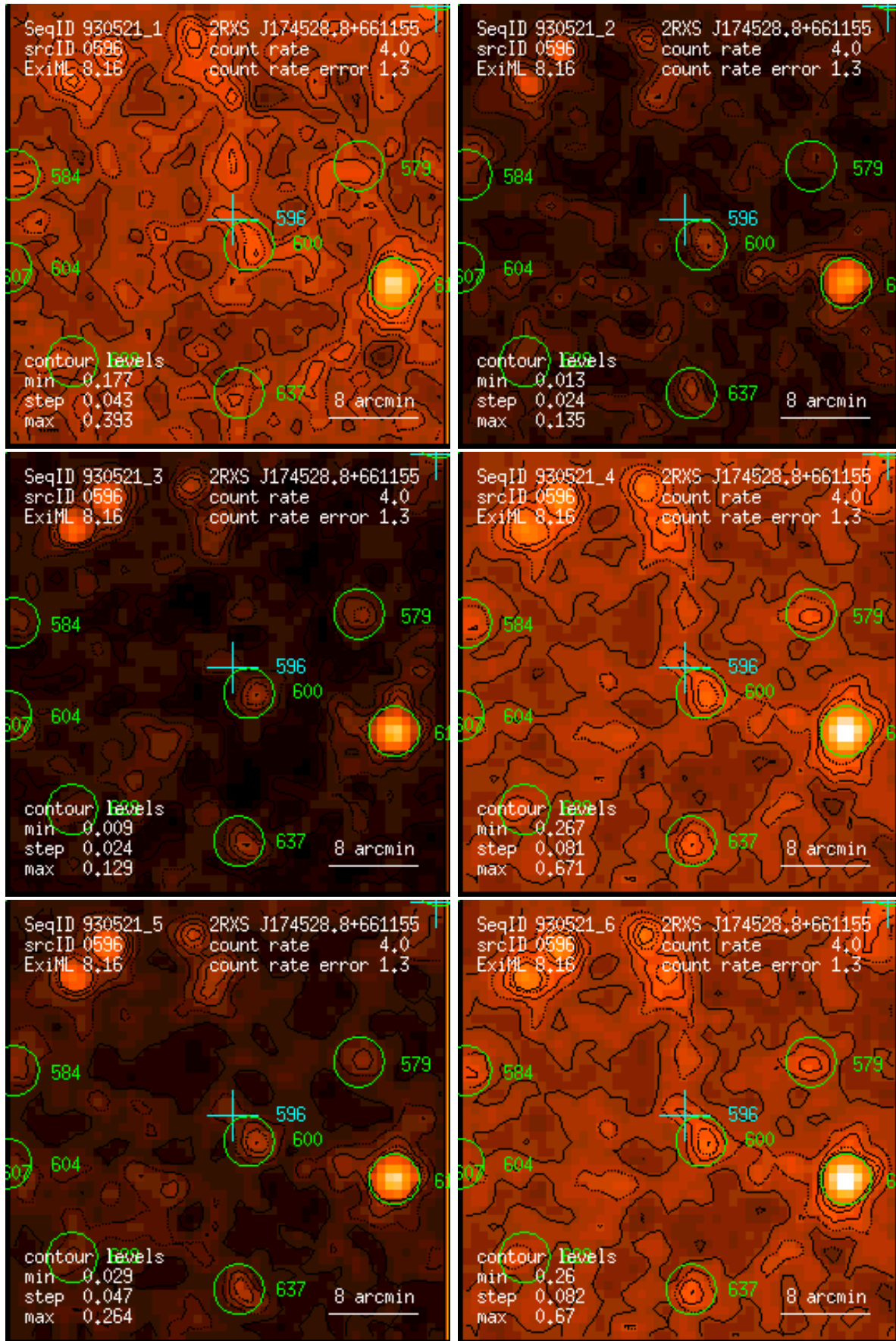
Figure 596: RASS 930521: detection 0596: band rate images, Gaussian filter: (1) PSPC channels 11 – 41, (2) 52 – 90, (3) 91 – 201, (4) 11 – 235, (5) 52 – 201, (6) 11 – 201. Broad band rates in counts/ks. Band rate contour levels in counts/ks/arcmin 2 .
