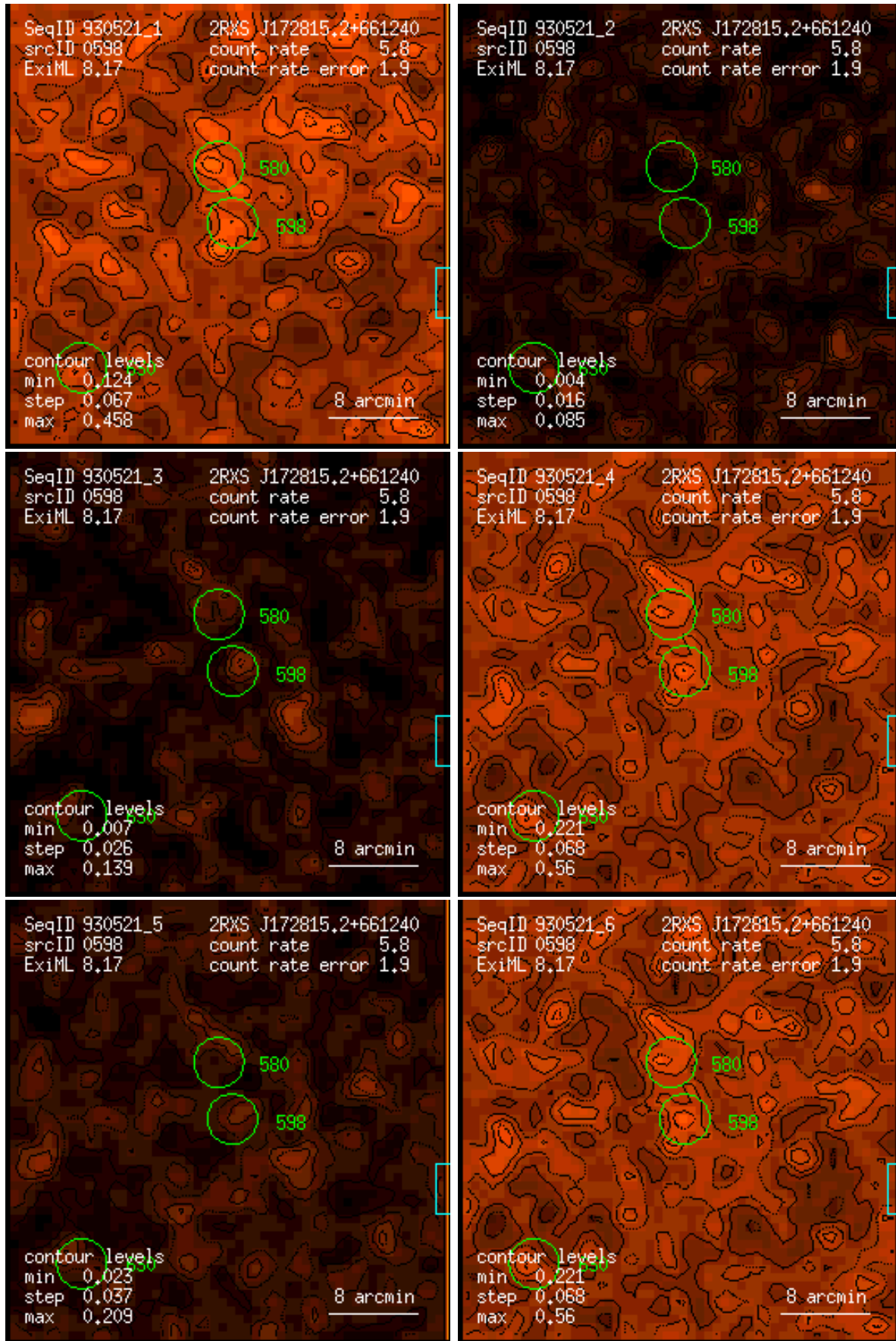
Figure 598: RASS 930521: detection 0598: band rate images, Gaussian filter: (1) PSPC channels 11 – 41, (2) 52 – 90, (3) 91 – 201, (4) 11 – 235, (5) 52 – 201, (6) 11 – 201. Broad band rates in counts/ks. Band rate contour levels in counts/ks/arcmin 2 .
