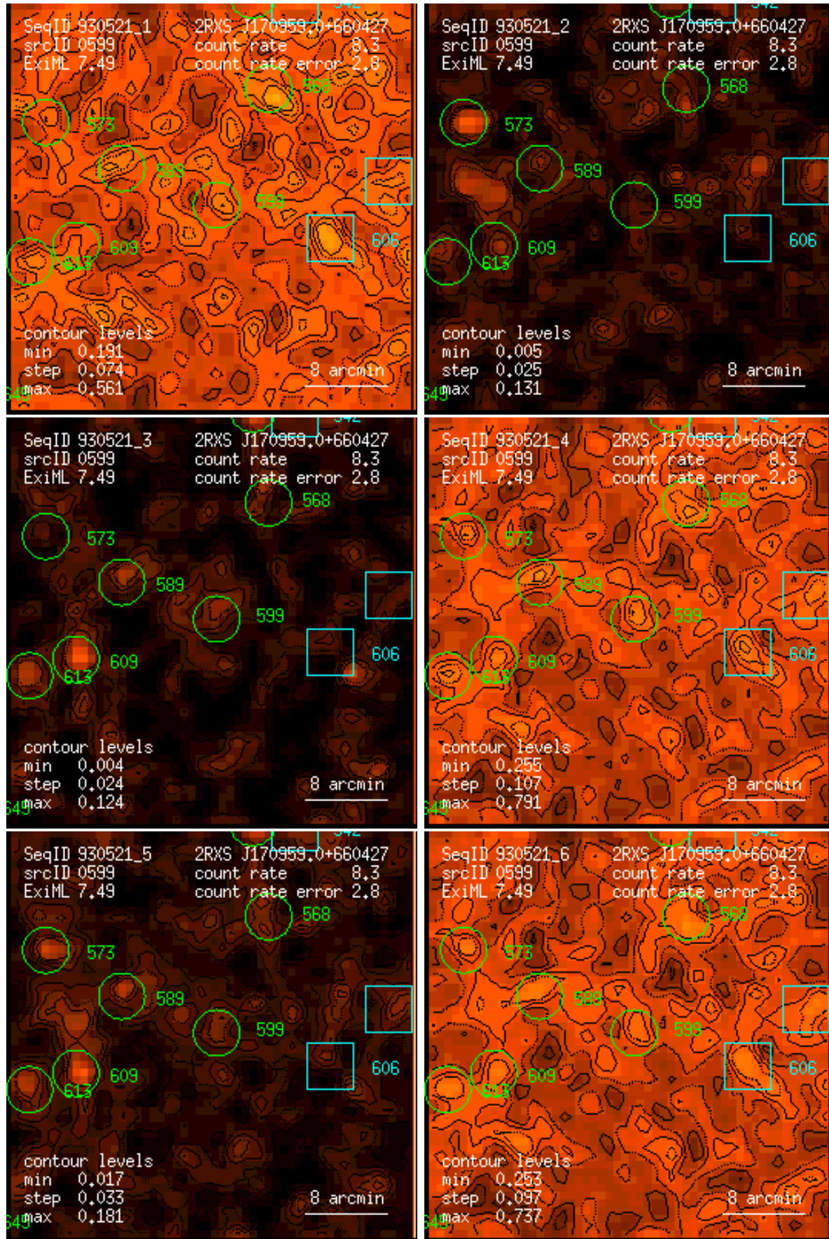
Figure 599: RASS 930521: detection 0599: band rate images, Gaussian filter: (1) PSPC channels 11 – 41, (2) 52 – 90, (3) 91 – 201, (4) 11 – 235, (5) 52 – 201, (6) 11 – 201. Broad band rates in counts/ks. Band rate contour levels in counts/ks/arcmin 2 .
