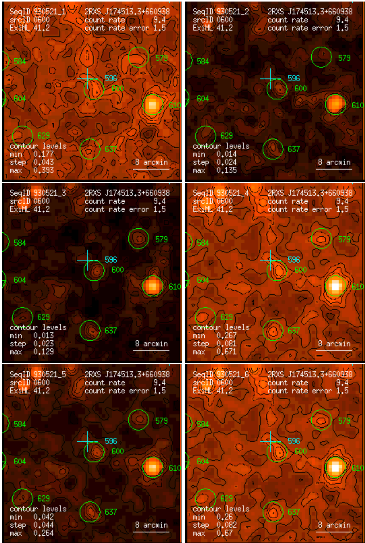
Figure 600: RASS 930521: detection 0600: band rate images, Gaussian filter: (1) PSPC channels 11 – 41, (2) 52 – 90, (3) 91 – 201, (4) 11 – 235, (5) 52 – 201, (6) 11 – 201. Broad band rates in counts/ks. Band rate contour levels in counts/ks/arcmin 2 .
