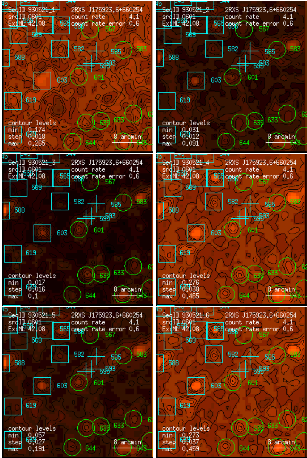
Figure 601: RASS 930521: detection 0601: band rate images, Gaussian filter: (1) PSPC channels 11 – 41, (2) 52 – 90, (3) 91 – 201, (4) 11 – 235, (5) 52 – 201, (6) 11 – 201. Broad band rates in counts/ks. Band rate contour levels in counts/ks/arcmin 2 .
