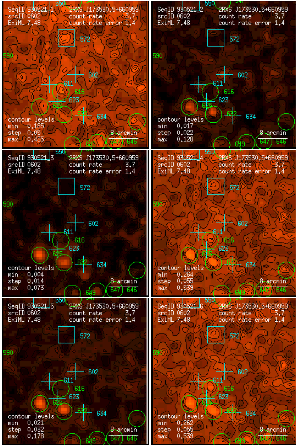
Figure 602: RASS 930521: detection 0602: band rate images, Gaussian filter: (1) PSPC channels 11 – 41, (2) 52 – 90, (3) 91 – 201, (4) 11 – 235, (5) 52 – 201, (6) 11 – 201. Broad band rates in counts/ks. Band rate contour levels in counts/ks/arcmin 2 .
