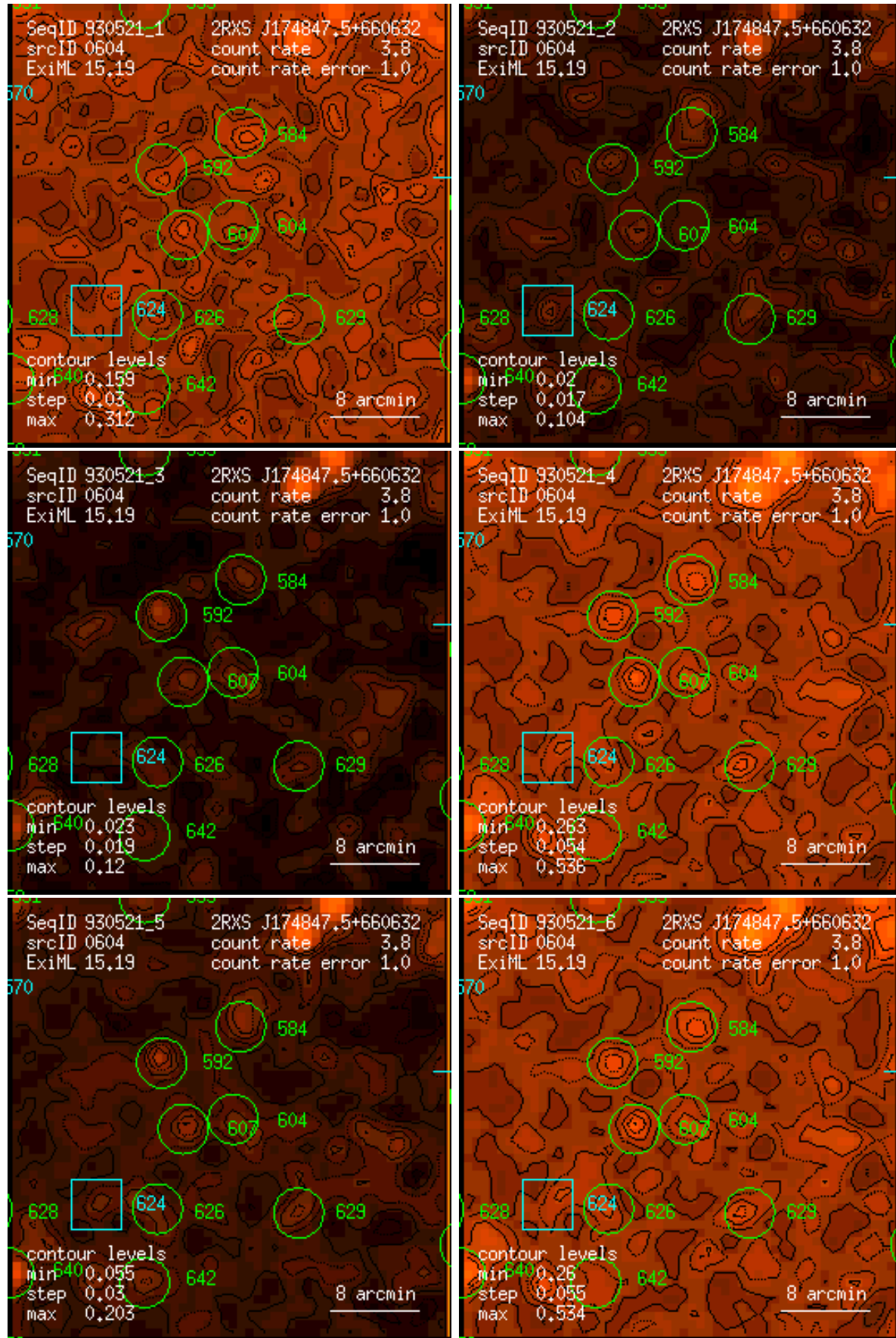
Figure 604: RASS 930521: detection 0604: band rate images, Gaussian filter: (1) PSPC channels 11 – 41, (2) 52 – 90, (3) 91 – 201, (4) 11 – 235, (5) 52 – 201, (6) 11 – 201. Broad band rates in counts/ks. Band rate contour levels in counts/ks/arcmin 2 .
