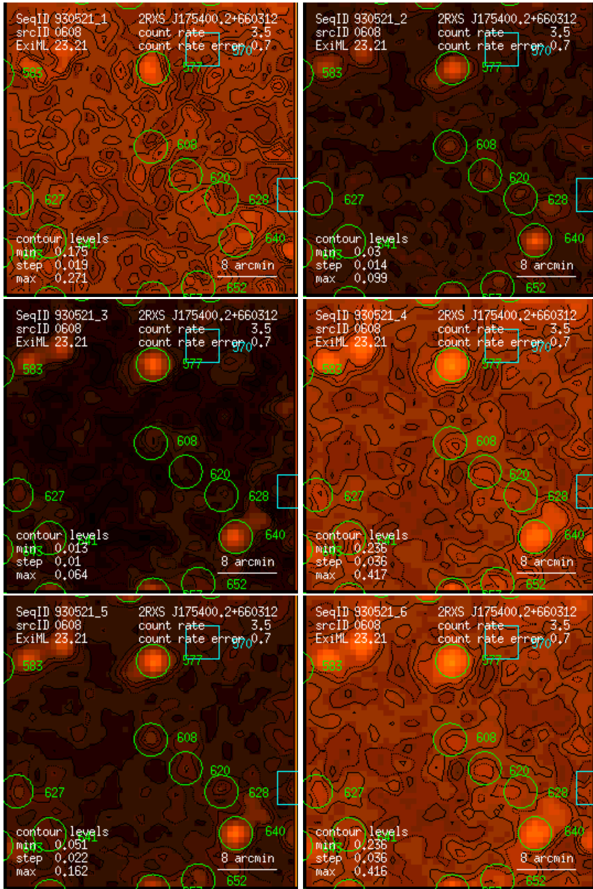
Figure 608: RASS 930521: detection 0608: band rate images, Gaussian filter: (1) PSPC channels 11 – 41, (2) 52 – 90, (3) 91 – 201, (4) 11 – 235, (5) 52 – 201, (6) 11 – 201. Broad band rates in counts/ks. Band rate contour levels in counts/ks/arcmin 2 .
