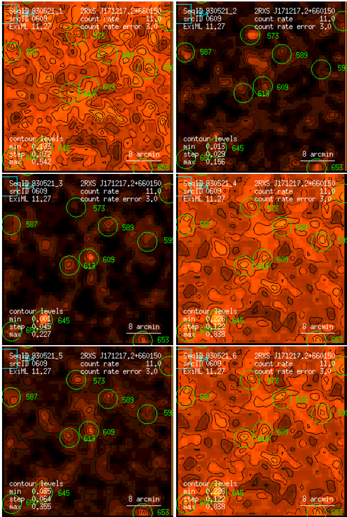
Figure 609: RASS 930521: detection 0609: band rate images, Gaussian filter: (1) PSPC channels 11 – 41, (2) 52 – 90, (3) 91 – 201, (4) 11 – 235, (5) 52 – 201, (6) 11 – 201. Broad band rates in counts/ks. Band rate contour levels in counts/ks/arcmin 2 .
