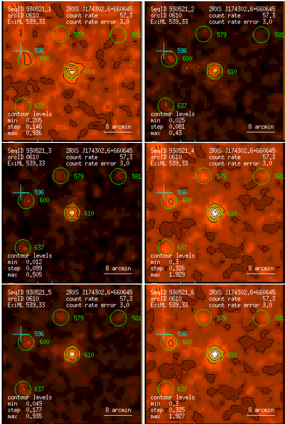
Figure 610: RASS 930521: detection 0610: band rate images, Gaussian filter: (1) PSPC channels 11 – 41, (2) 52 – 90, (3) 91 – 201, (4) 11 – 235, (5) 52 – 201, (6) 11 – 201. Broad band rates in counts/ks. Band rate contour levels in counts/ks/arcmin 2 .
