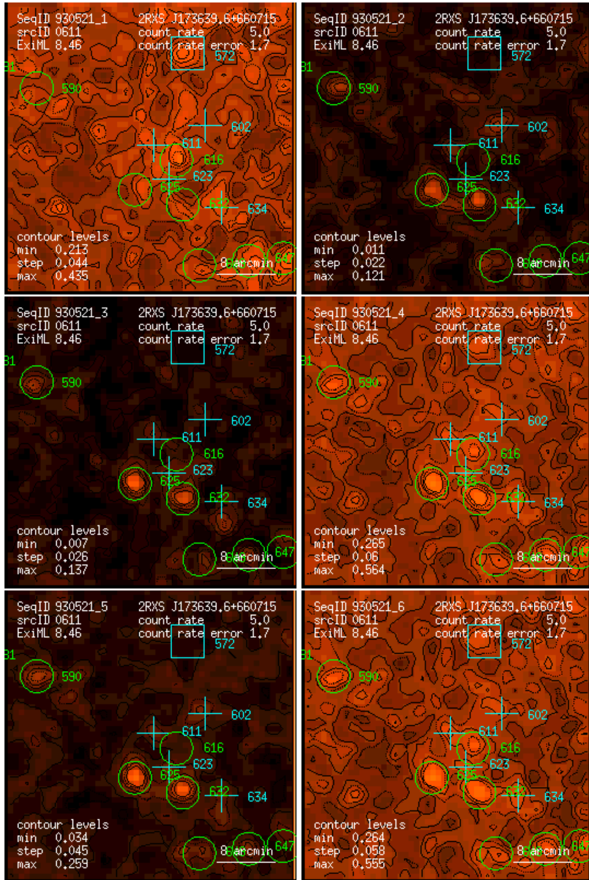
Figure 611: RASS 930521: detection 0611: band rate images, Gaussian filter: (1) PSPC channels 11 – 41, (2) 52 – 90, (3) 91 – 201, (4) 11 – 235, (5) 52 – 201, (6) 11 – 201. Broad band rates in counts/ks. Band rate contour levels in counts/ks/arcmin 2 .
