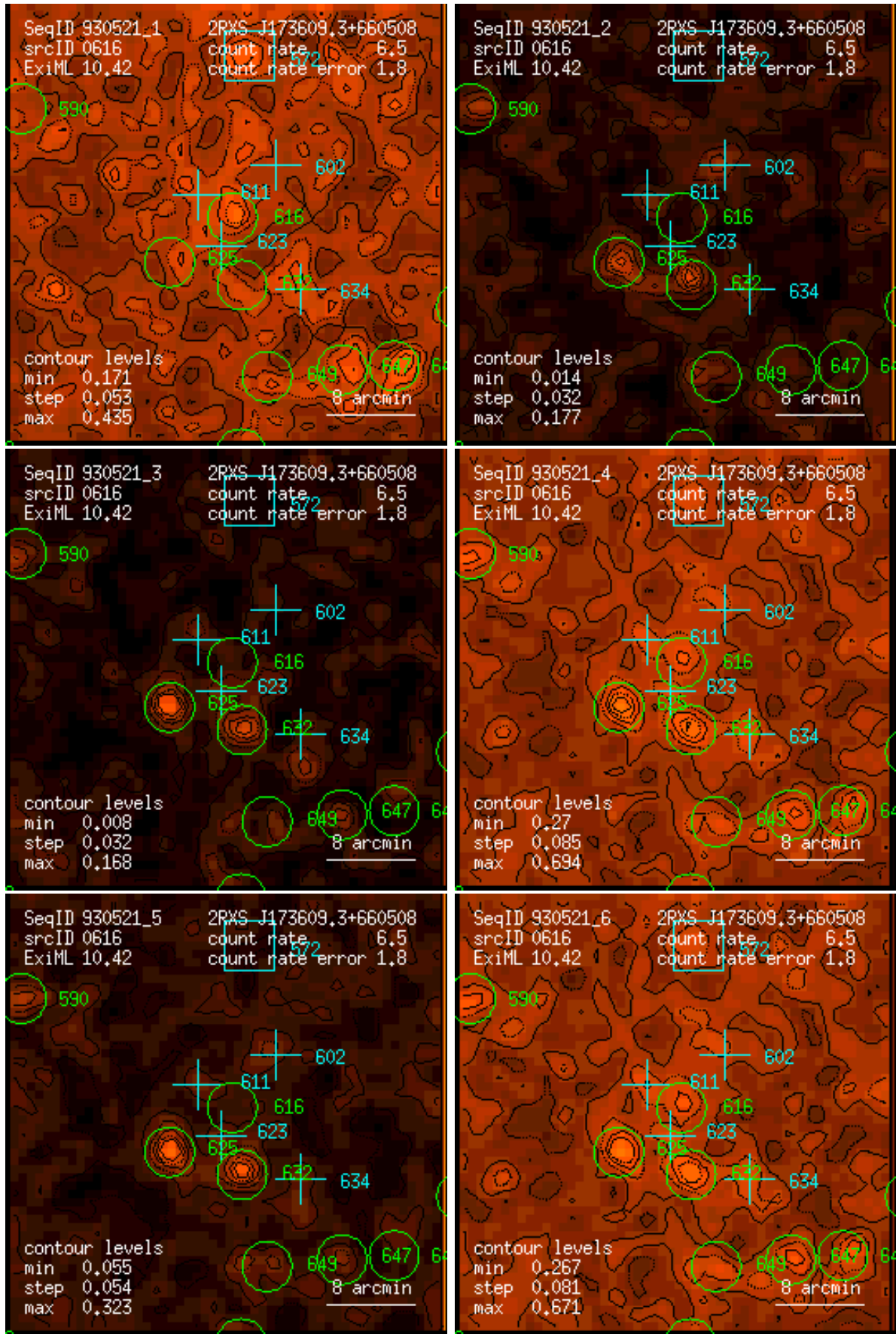
Figure 616: RASS 930521: detection 0616: band rate images, Gaussian filter: (1) PSPC channels 11 – 41, (2) 52 – 90, (3) 91 – 201, (4) 11 – 235, (5) 52 – 201, (6) 11 – 201. Broad band rates in counts/ks. Band rate contour levels in counts/ks/arcmin 2 .
