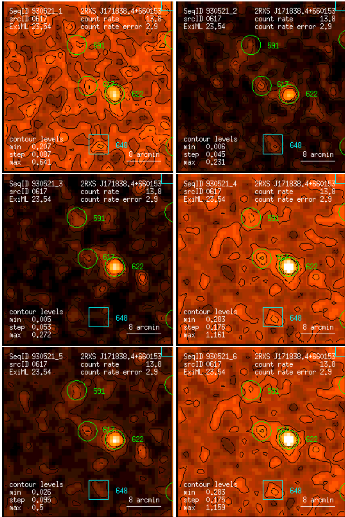
Figure 617: RASS 930521: detection 0617: band rate images, Gaussian filter: (1) PSPC channels 11 – 41, (2) 52 – 90, (3) 91 – 201, (4) 11 – 235, (5) 52 – 201, (6) 11 – 201. Broad band rates in counts/ks. Band rate contour levels in counts/ks/arcmin 2 .
